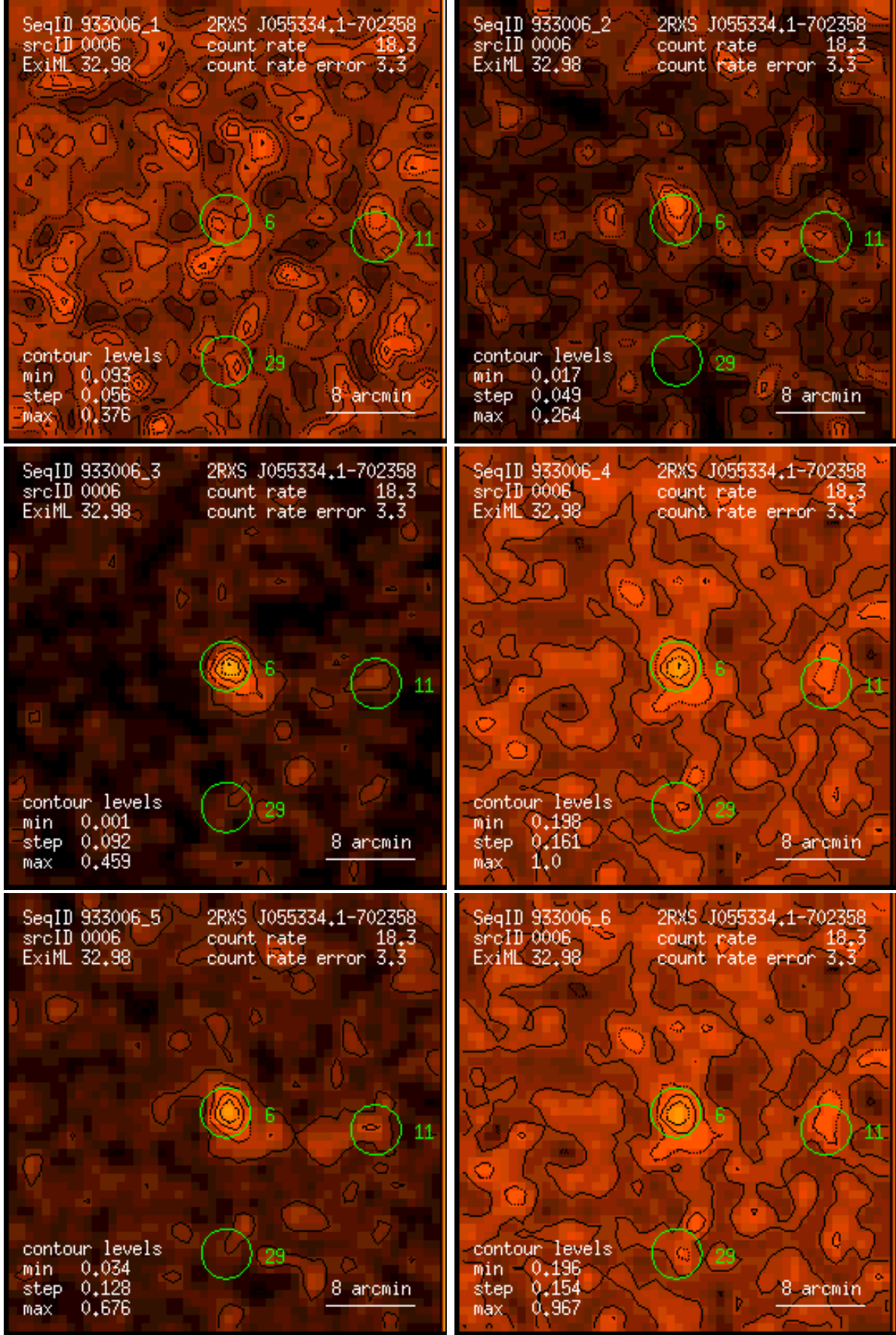
Figure 6: RASS 933006: detection 0006: band rate images, Gaussian filter: (1) PSPC channels 11 – 41, (2) 52 – 90, (3) 91 – 201, (4) 11 – 235, (5) 52 – 201, (6) 11 – 201. Broad band rates in counts/ks. Band rate contour levels in counts/ks/arcmin 2 .
