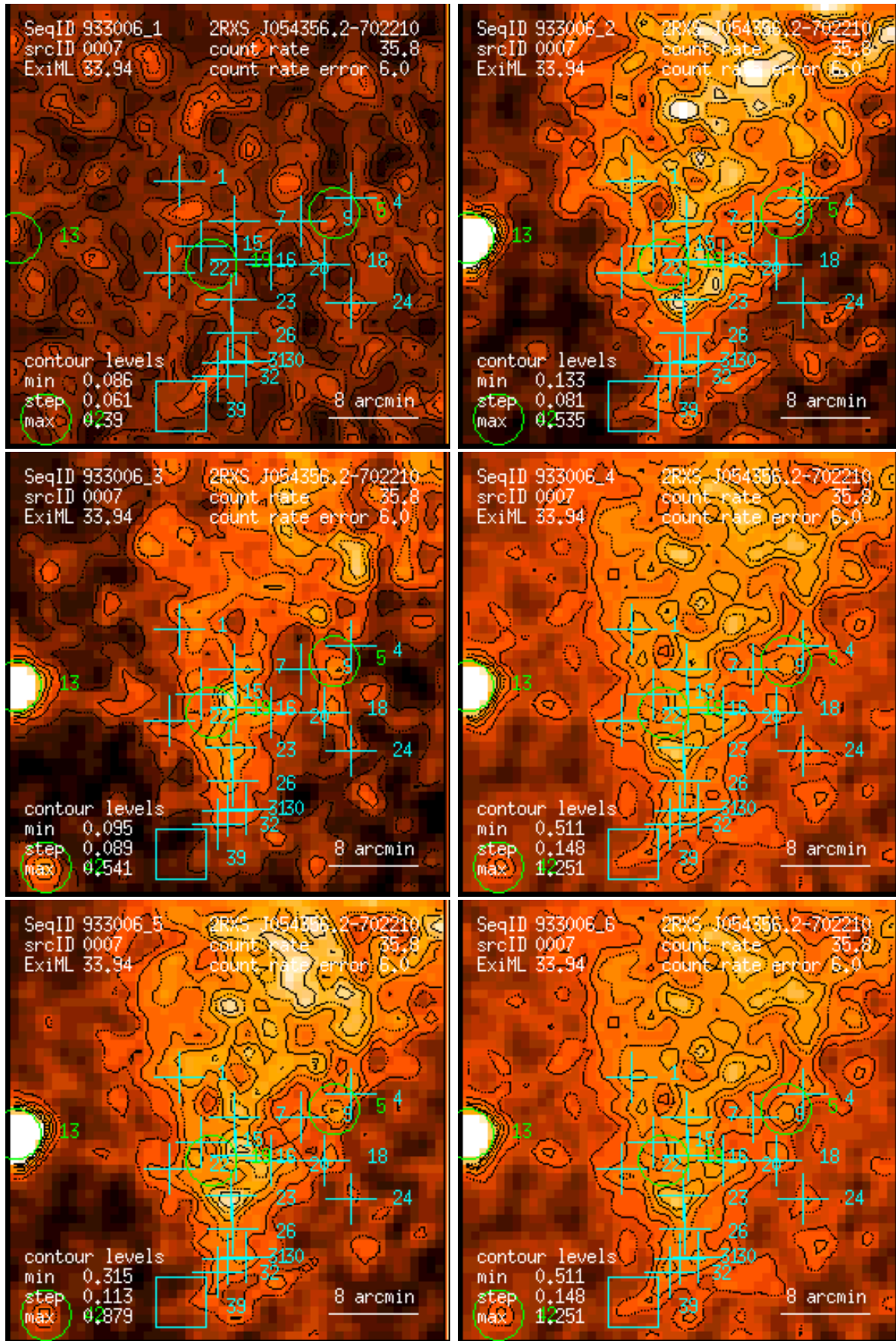
Figure 7: RASS 933006: detection 0007: band rate images, Gaussian filter: (1) PSPC channels 11 – 41, (2) 52 – 90, (3) 91 – 201, (4) 11 – 235, (5) 52 – 201, (6) 11 – 201. Broad band rates in counts/ks. Band rate contour levels in counts/ks/arcmin 2 .
