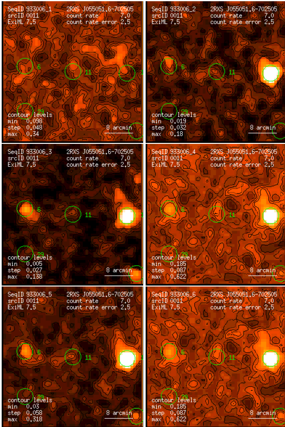
Figure 11: RASS 933006: detection 0011: band rate images, Gaussian filter: (1) PSPC channels 11 – 41, (2) 52 – 90, (3) 91 – 201, (4) 11 – 235, (5) 52 – 201, (6) 11 – 201. Broad band rates in counts/ks. Band rate contour levels in counts/ks/arcmin 2 .
