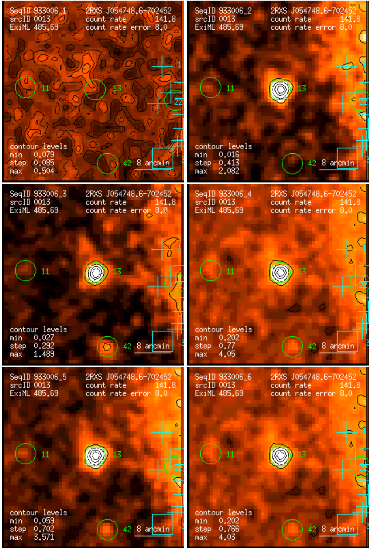
Figure 13: RASS 933006: detection 0013: band rate images, Gaussian filter: (1) PSPC channels 11 – 41, (2) 52 – 90, (3) 91 – 201, (4) 11 – 235, (5) 52 – 201, (6) 11 – 201. Broad band rates in counts/ks. Band rate contour levels in counts/ks/arcmin 2 .
