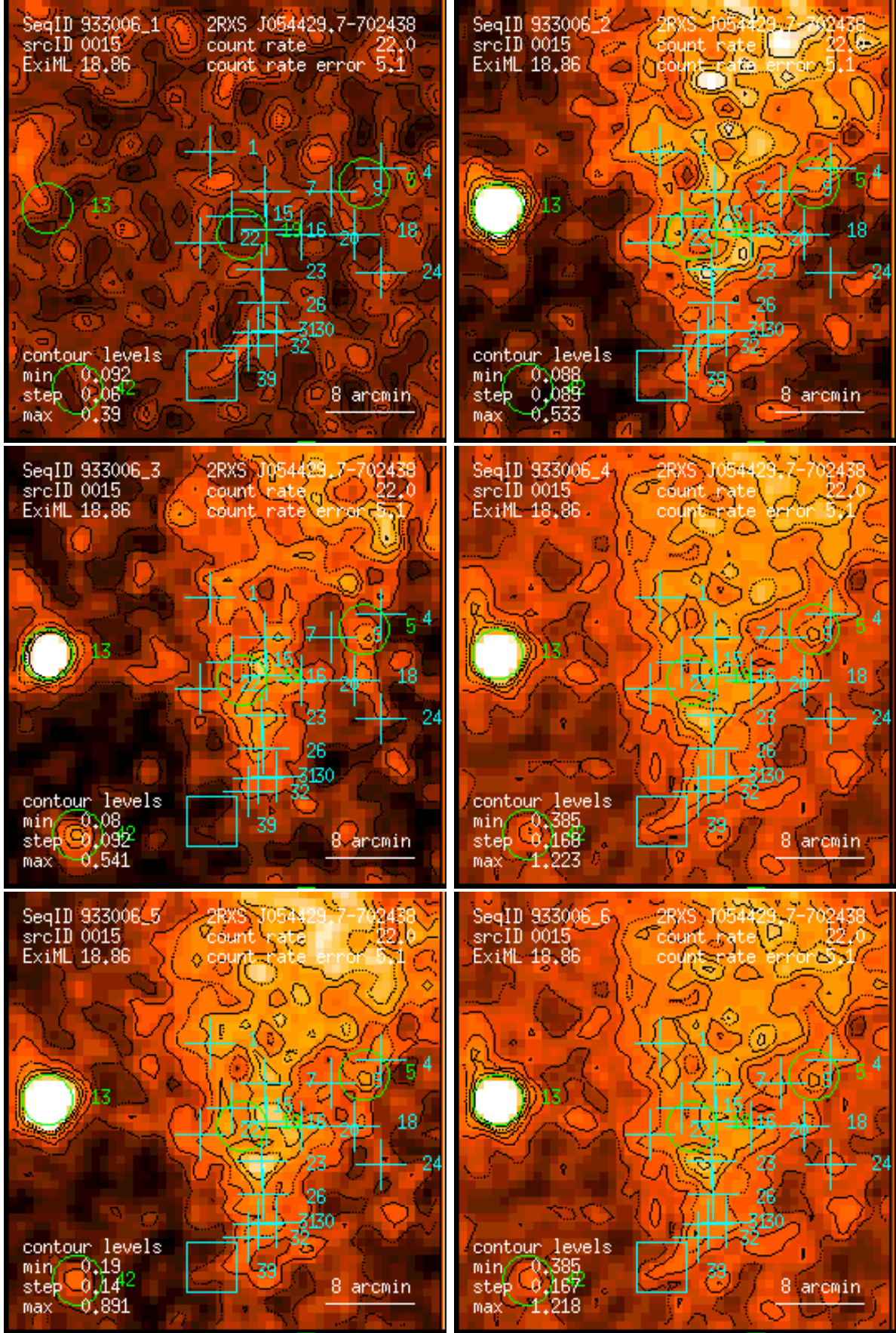
Figure 15: RASS 933006: detection 0015: band rate images, Gaussian filter: (1) PSPC channels 11 – 41, (2) 52 – 90, (3) 91 – 201, (4) 11 – 235, (5) 52 – 201, (6) 11 – 201. Broad band rates in counts/ks. Band rate contour levels in counts/ks/arcmin 2 .
