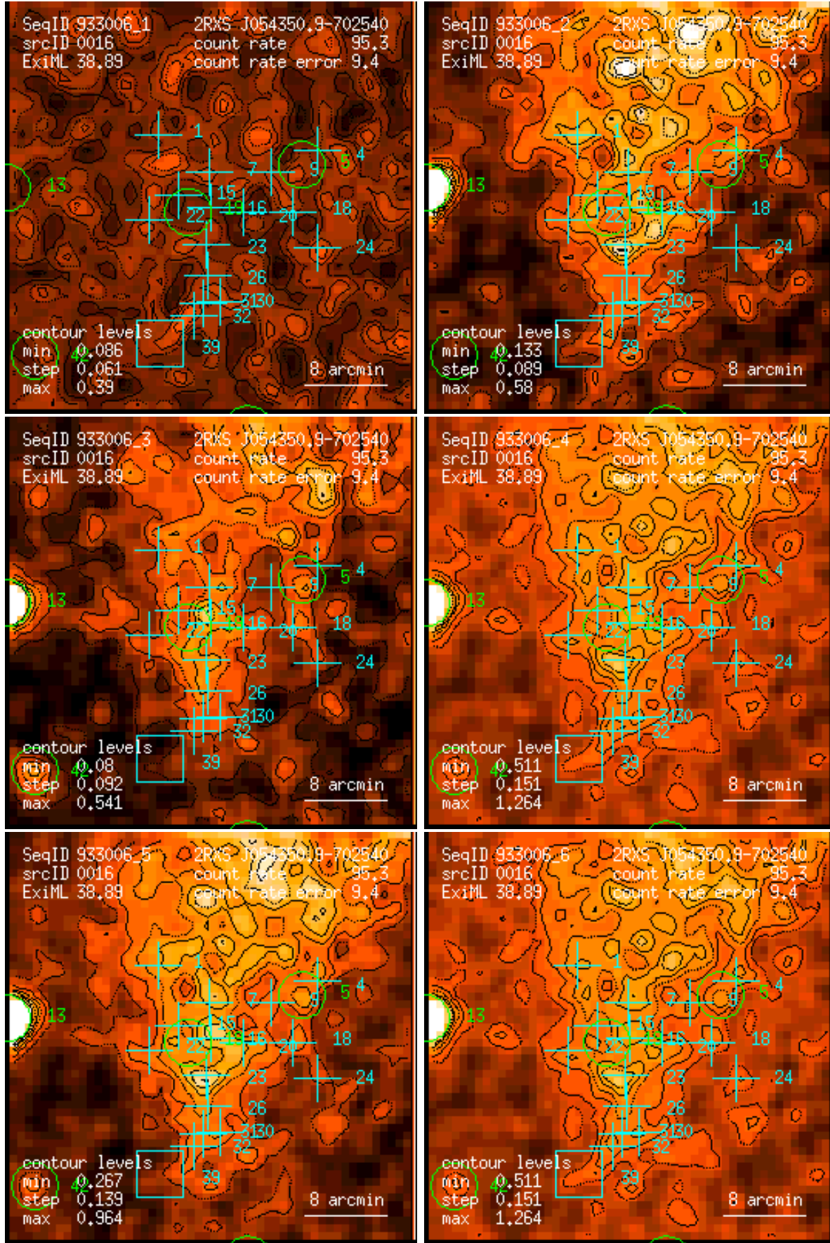
Figure 16: RASS 933006: detection 0016: band rate images, Gaussian filter: (1) PSPC channels 11 – 41, (2) 52 – 90, (3) 91 – 201, (4) 11 – 235, (5) 52 – 201, (6) 11 – 201. Broad band rates in counts/ks. Band rate contour levels in counts/ks/arcmin 2 .
