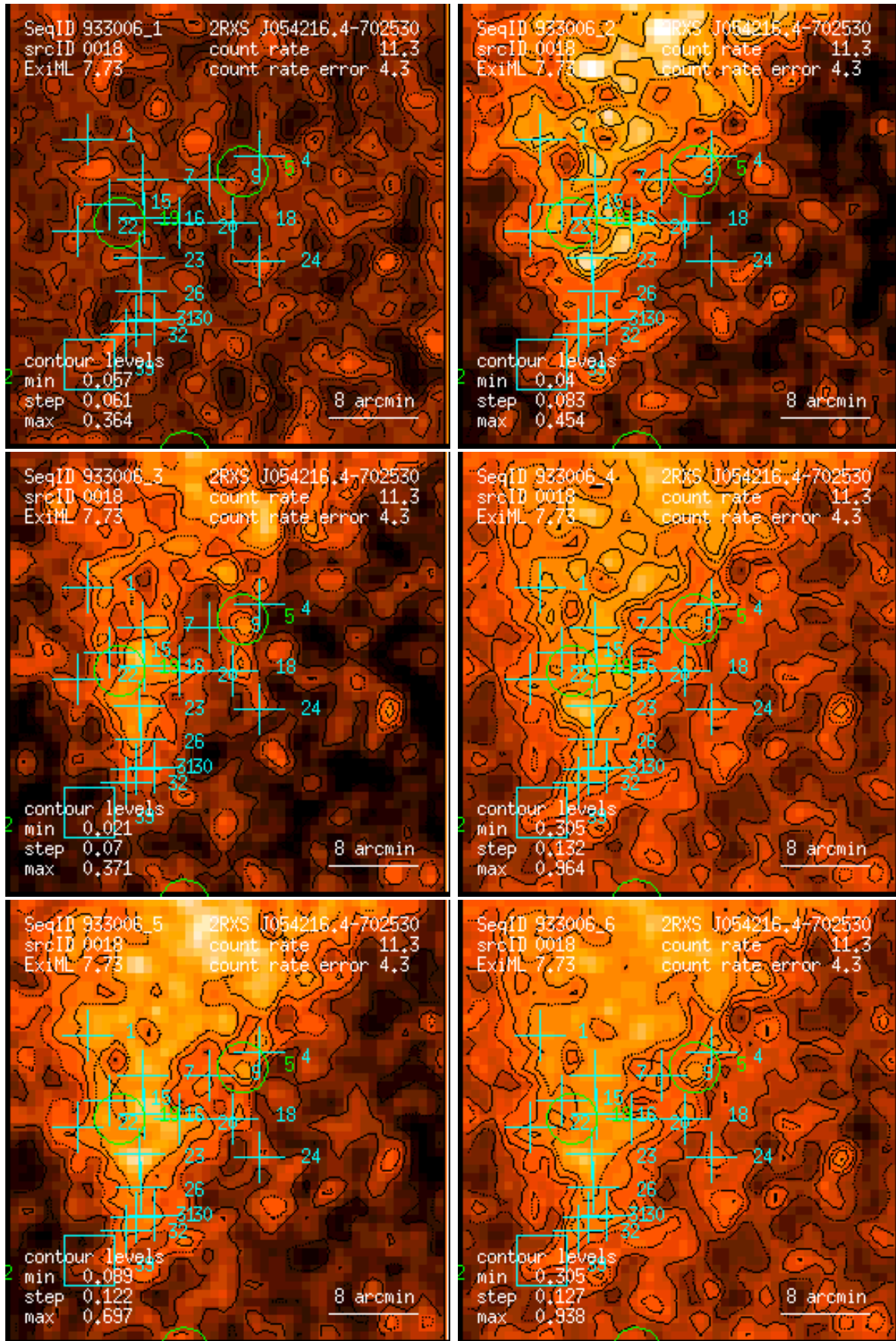
Figure 18: RASS 933006: detection 0018: band rate images, Gaussian filter: (1) PSPC channels 11 – 41, (2) 52 – 90, (3) 91 – 201, (4) 11 – 235, (5) 52 – 201, (6) 11 – 201. Broad band rates in counts/ks. Band rate contour levels in counts/ks/arcmin 2 .
