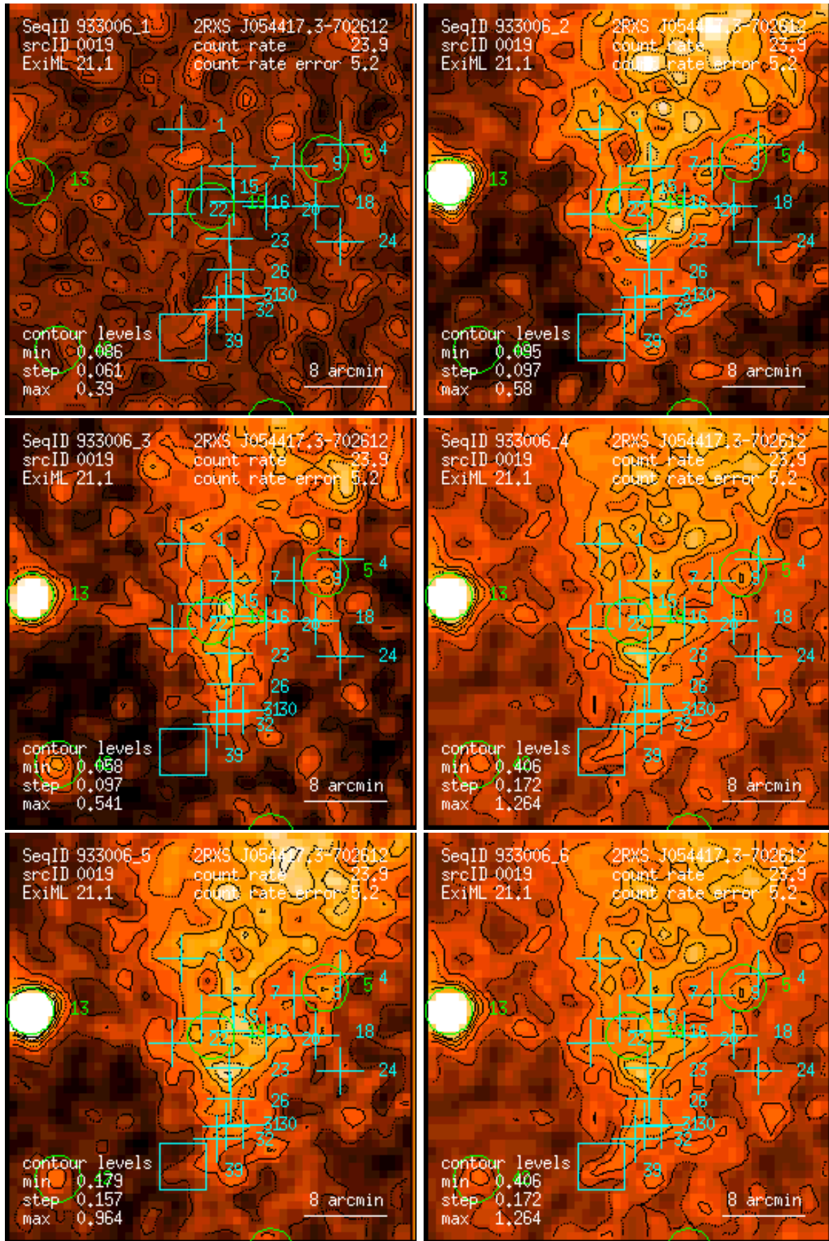
Figure 19: RASS 933006: detection 0019: band rate images, Gaussian filter: (1) PSPC channels 11 – 41, (2) 52 – 90, (3) 91 – 201, (4) 11 – 235, (5) 52 – 201, (6) 11 – 201. Broad band rates in counts/ks. Band rate contour levels in counts/ks/arcmin 2 .
