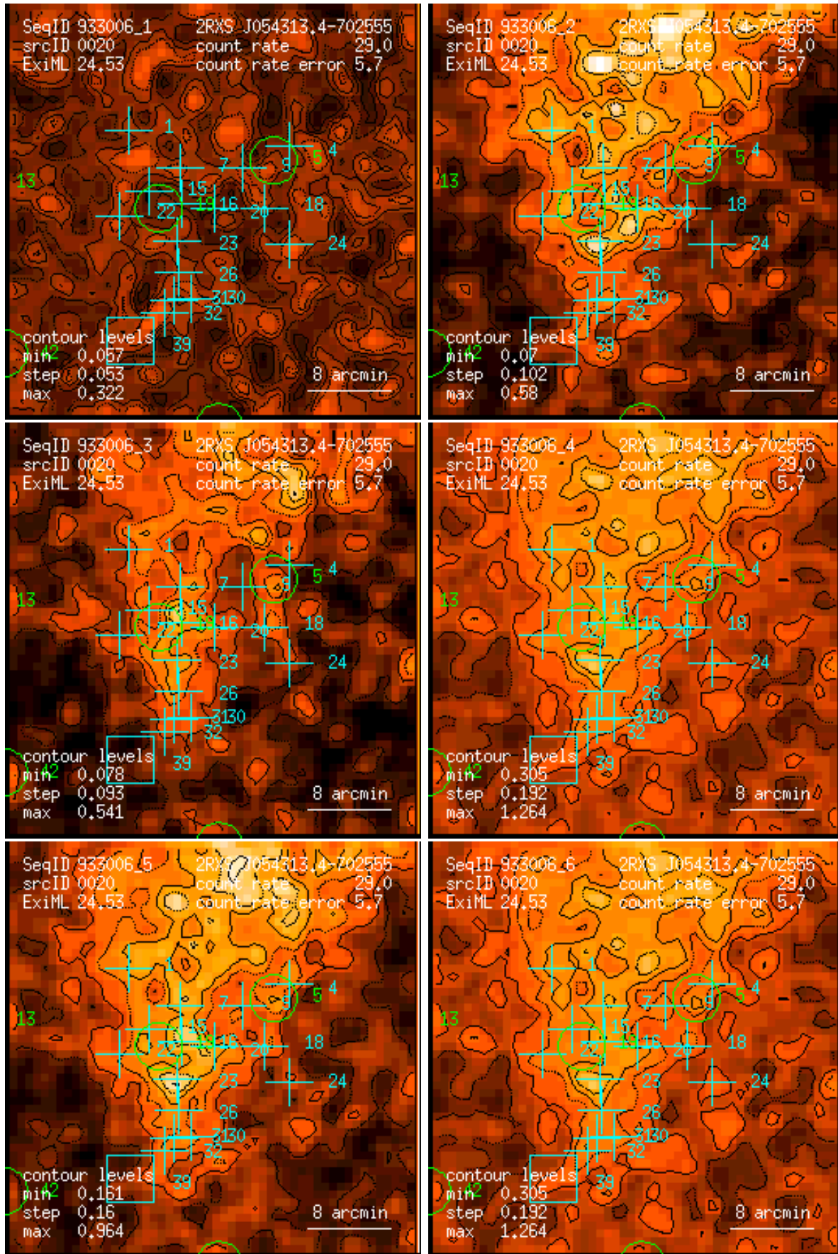
Figure 20: RASS 933006: detection 0020: band rate images, Gaussian filter: (1) PSPC channels 11 – 41, (2) 52 – 90, (3) 91 – 201, (4) 11 – 235, (5) 52 – 201, (6) 11 – 201. Broad band rates in counts/ks. Band rate contour levels in counts/ks/arcmin 2 .
