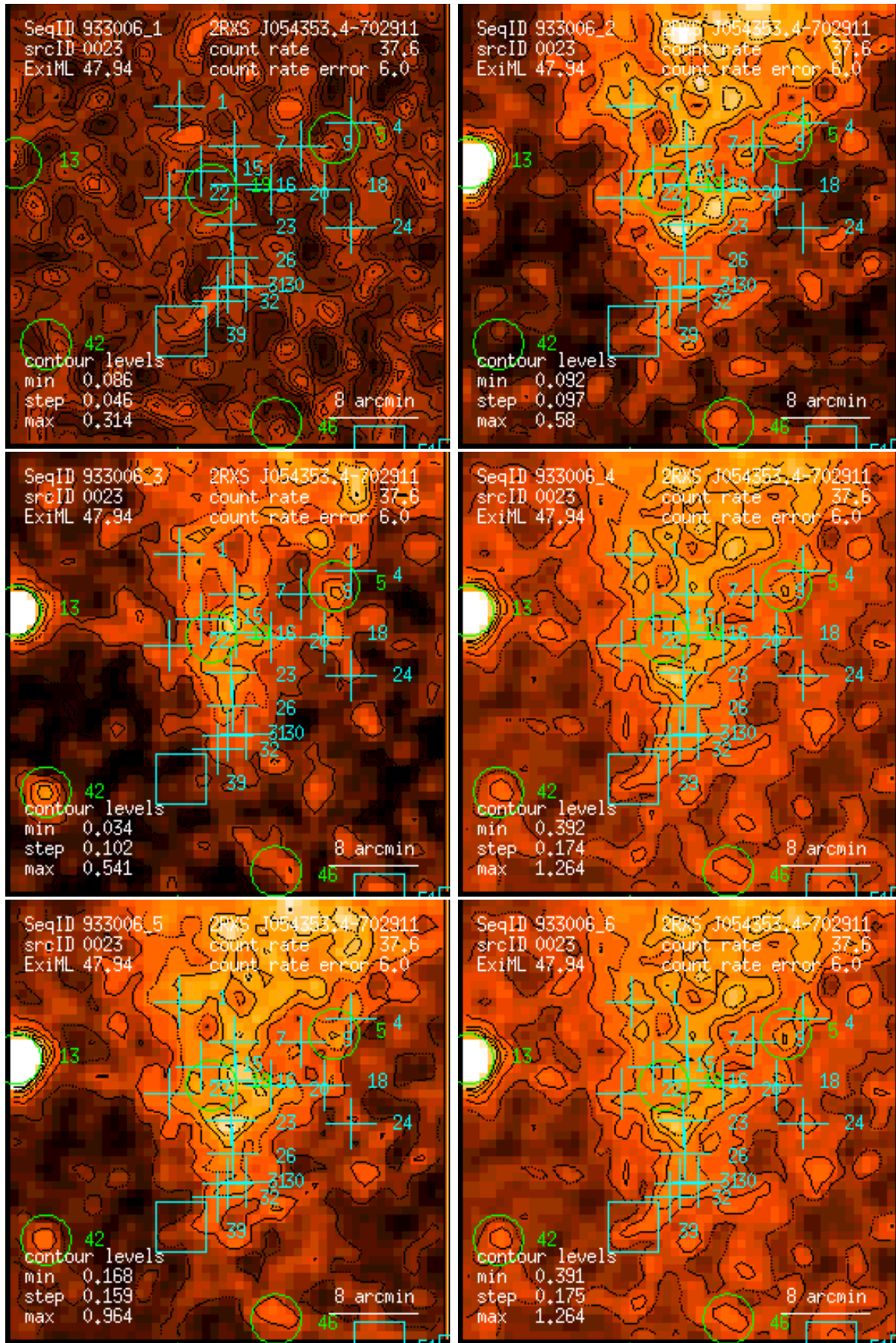
Figure 23: RASS 933006: detection 0023: band rate images, Gaussian filter: (1) PSPC channels 11 – 41, (2) 52 – 90, (3) 91 – 201, (4) 11 – 235, (5) 52 – 201, (6) 11 – 201. Broad band rates in counts/ks. Band rate contour levels in counts/ks/arcmin 2 .
