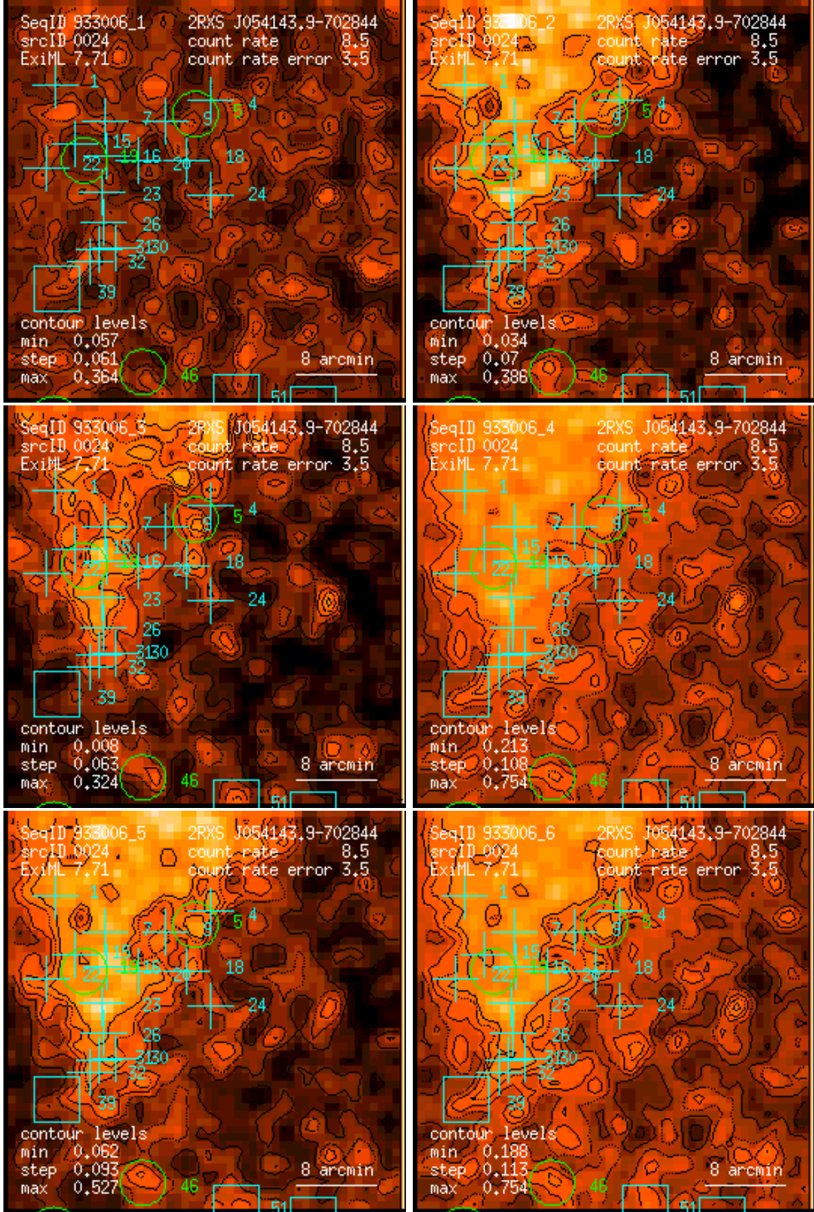
Figure 24: RASS 933006: detection 0024: band rate images, Gaussian filter: (1) PSPC channels 11 – 41, (2) 52 – 90, (3) 91 – 201, (4) 11 – 235, (5) 52 – 201, (6) 11 – 201. Broad band rates in counts/ks. Band rate contour levels in counts/ks/arcmin 2 .
