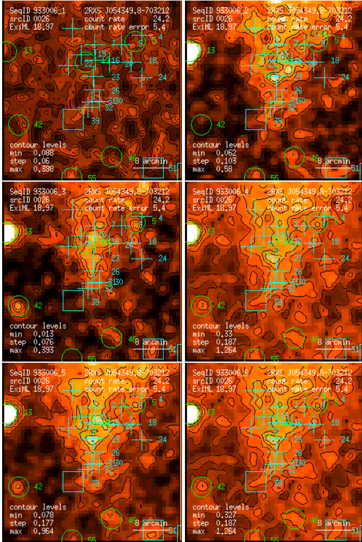
Figure 26: RASS 933006: detection 0026: band rate images, Gaussian filter: (1) PSPC channels 11 – 41, (2) 52 – 90, (3) 91 – 201, (4) 11 – 235, (5) 52 – 201, (6) 11 – 201. Broad band rates in counts/ks. Band rate contour levels in counts/ks/arcmin 2 .
