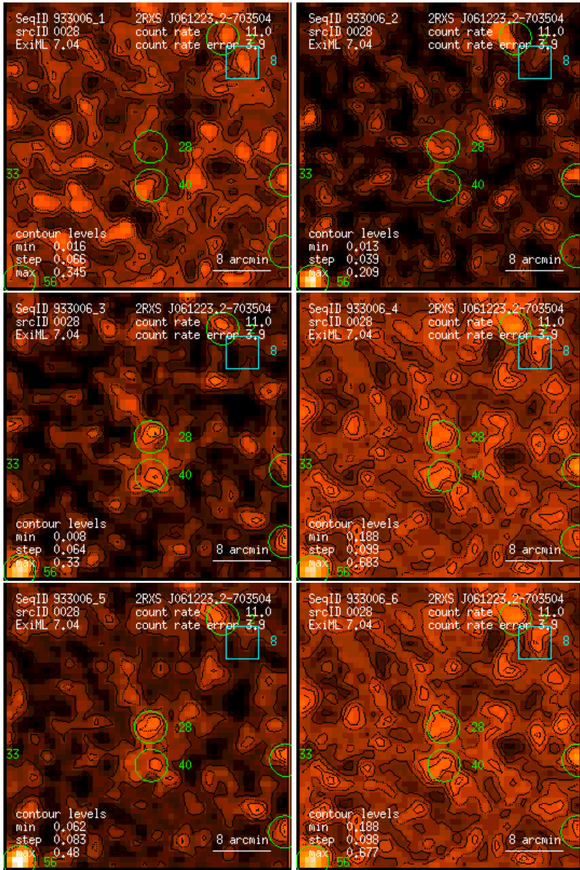
Figure 28: RASS 933006: detection 0028: band rate images, Gaussian filter: (1) PSPC channels 11 – 41, (2) 52 – 90, (3) 91 – 201, (4) 11 – 235, (5) 52 – 201, (6) 11 – 201. Broad band rates in counts/ks. Band rate contour levels in counts/ks/arcmin 2 .
