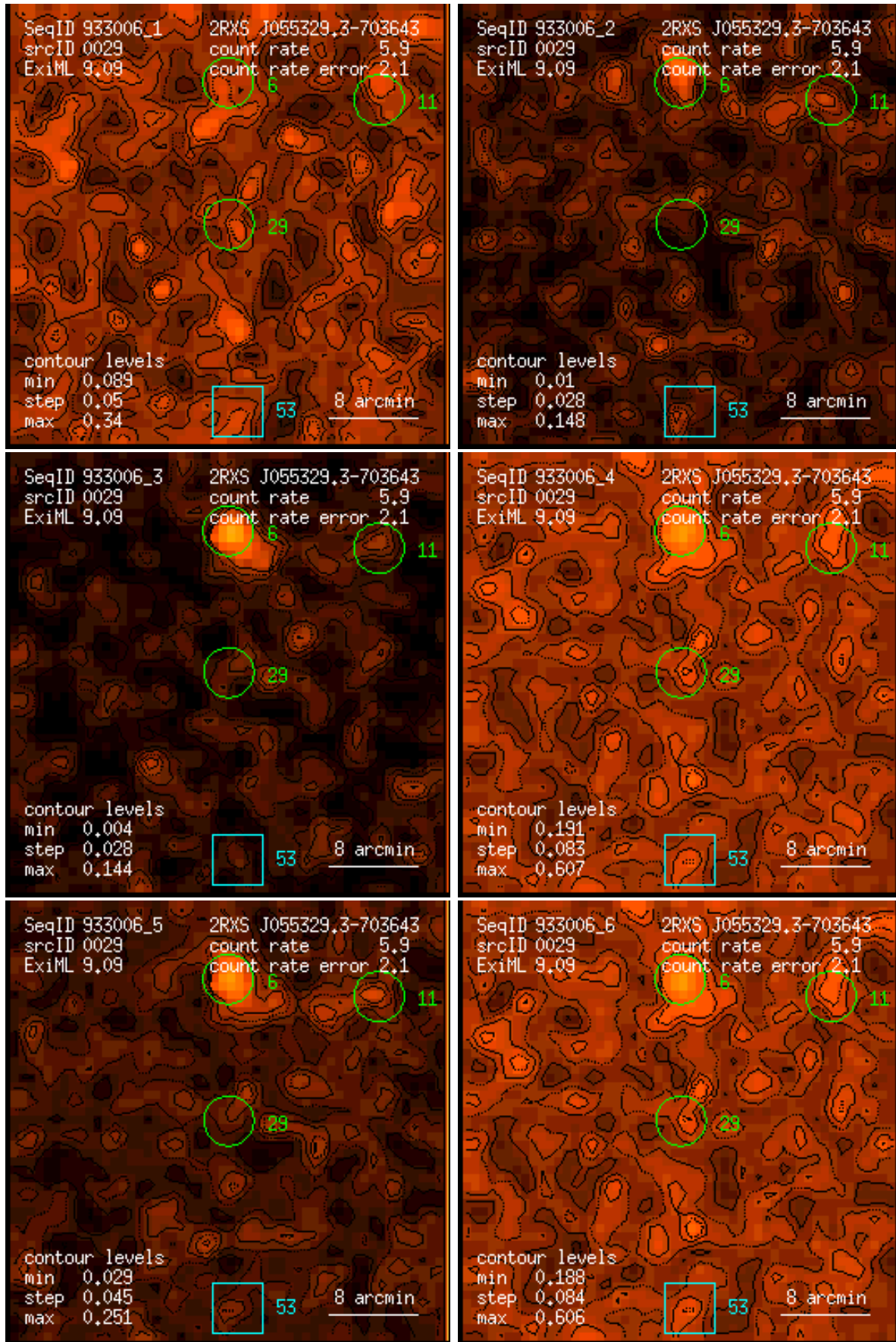
Figure 29: RASS 933006: detection 0029: band rate images, Gaussian filter: (1) PSPC channels 11 – 41, (2) 52 – 90, (3) 91 – 201, (4) 11 – 235, (5) 52 – 201, (6) 11 – 201. Broad band rates in counts/ks. Band rate contour levels in counts/ks/arcmin 2 .
