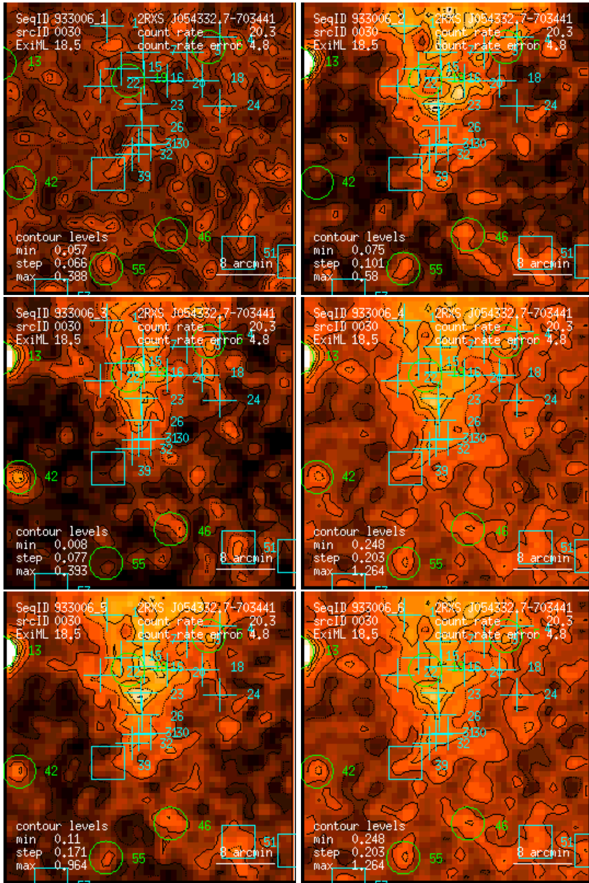
Figure 30: RASS 933006: detection 0030: band rate images, Gaussian filter: (1) PSPC channels 11 – 41, (2) 52 – 90, (3) 91 – 201, (4) 11 – 235, (5) 52 – 201, (6) 11 – 201. Broad band rates in counts/ks. Band rate contour levels in counts/ks/arcmin 2 .
