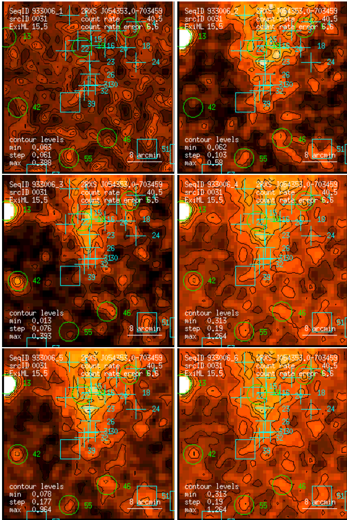
Figure 31: RASS 933006: detection 0031: band rate images, Gaussian filter: (1) PSPC channels 11 – 41, (2) 52 – 90, (3) 91 – 201, (4) 11 – 235, (5) 52 – 201, (6) 11 – 201. Broad band rates in counts/ks. Band rate contour levels in counts/ks/arcmin 2 .
