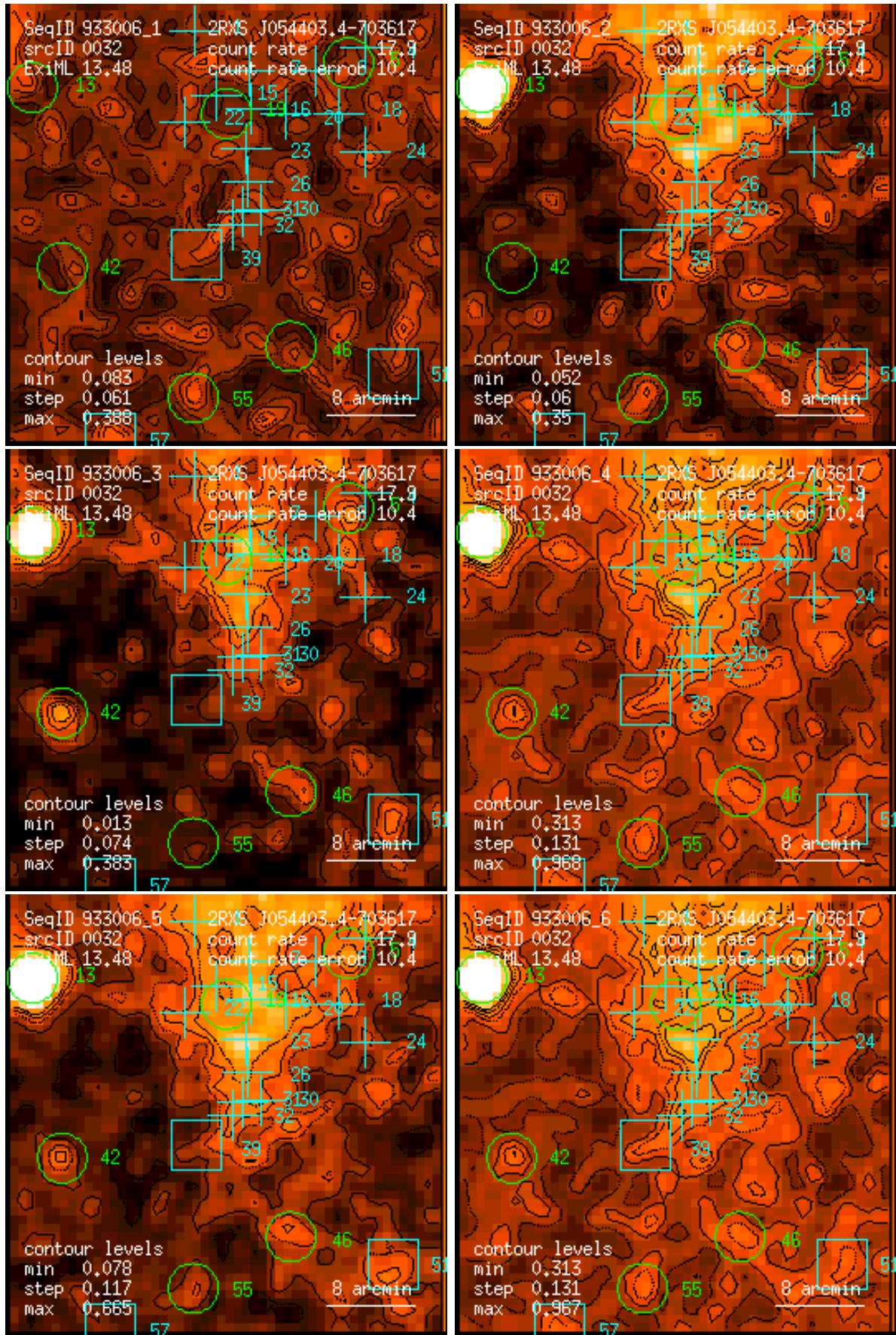
Figure 32: RASS 933006: detection 0032: band rate images, Gaussian filter: (1) PSPC channels 11 – 41, (2) 52 – 90, (3) 91 – 201, (4) 11 – 235, (5) 52 – 201, (6) 11 – 201. Broad band rates in counts/ks. Band rate contour levels in counts/ks/arcmin 2 .
