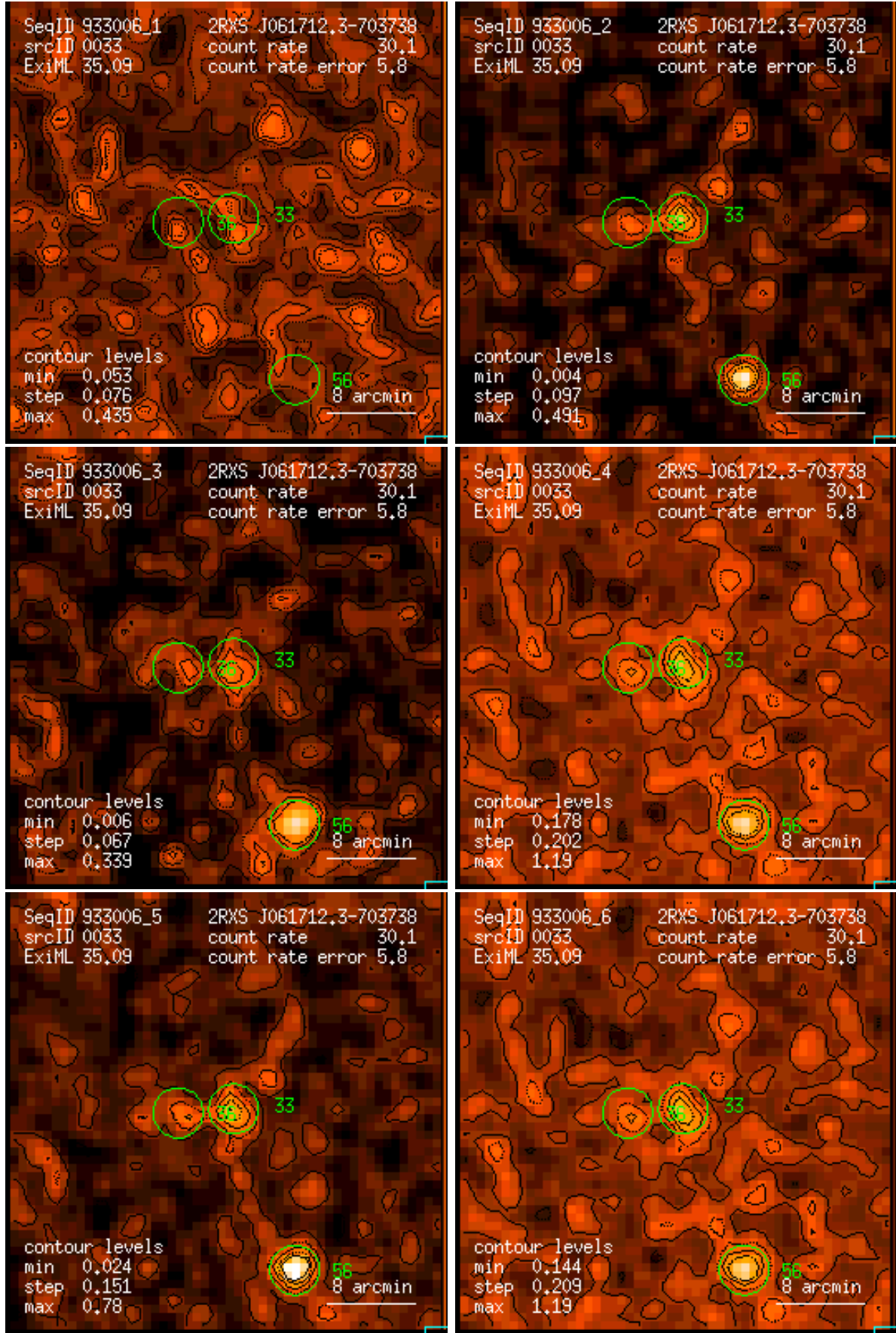
Figure 33: RASS 933006: detection 0033: band rate images, Gaussian filter: (1) PSPC channels 11 – 41, (2) 52 – 90, (3) 91 – 201, (4) 11 – 235, (5) 52 – 201, (6) 11 – 201. Broad band rates in counts/ks. Band rate contour levels in counts/ks/arcmin 2 .
