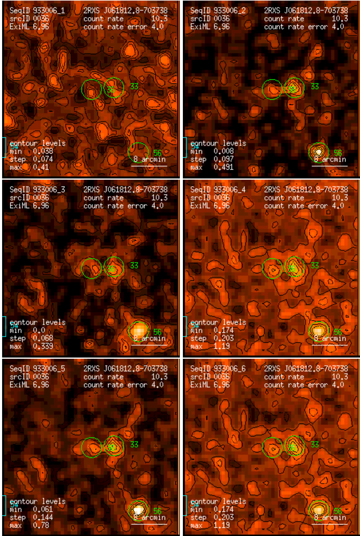
Figure 36: RASS 933006: detection 0036: band rate images, Gaussian filter: (1) PSPC channels 11 – 41, (2) 52 – 90, (3) 91 – 201, (4) 11 – 235, (5) 52 – 201, (6) 11 – 201. Broad band rates in counts/ks. Band rate contour levels in counts/ks/arcmin 2 .
