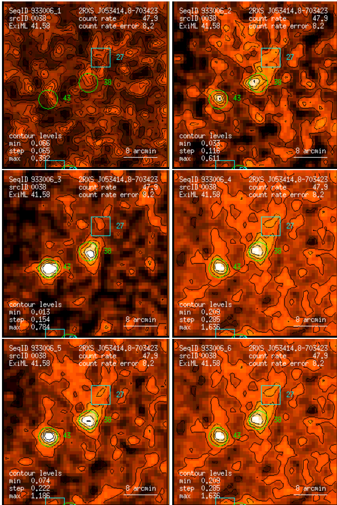
Figure 38: RASS 933006: detection 0038: band rate images, Gaussian filter: (1) PSPC channels 11 – 41, (2) 52 – 90, (3) 91 – 201, (4) 11 – 235, (5) 52 – 201, (6) 11 – 201. Broad band rates in counts/ks. Band rate contour levels in counts/ks/arcmin 2 .
