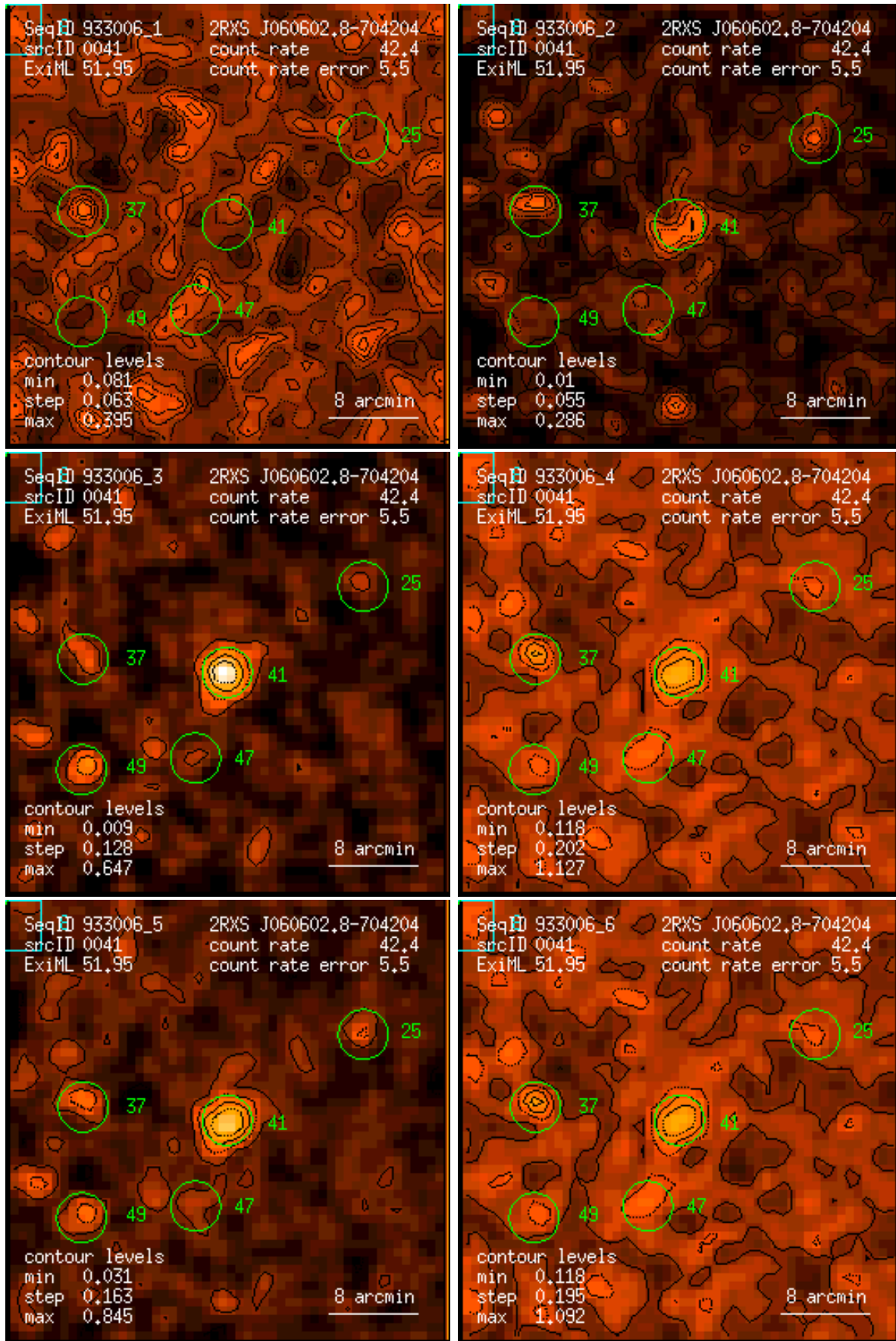
Figure 41: RASS 933006: detection 0041: band rate images, Gaussian filter: (1) PSPC channels 11 – 41, (2) 52 – 90, (3) 91 – 201, (4) 11 – 235, (5) 52 – 201, (6) 11 – 201. Broad band rates in counts/ks. Band rate contour levels in counts/ks/arcmin 2 .
