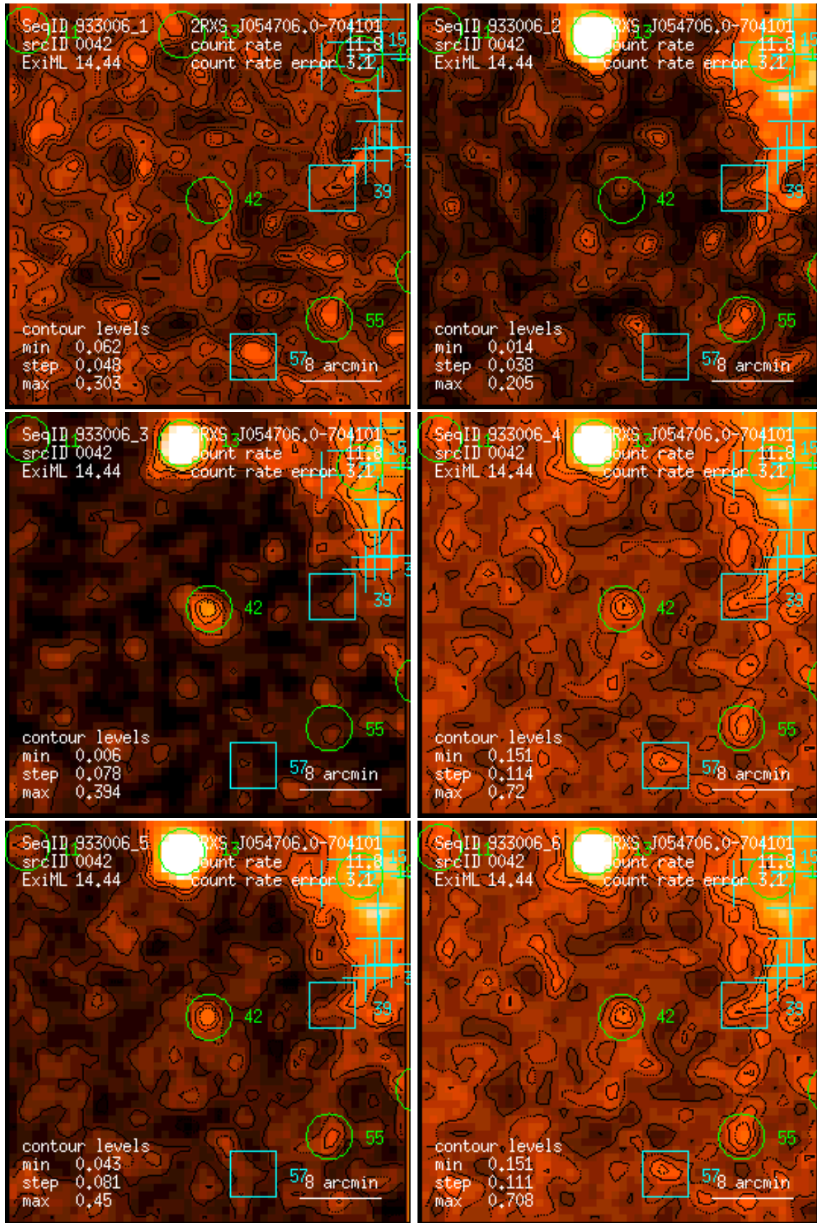
Figure 42: RASS 933006: detection 0042: band rate images, Gaussian filter: (1) PSPC channels 11 – 41, (2) 52 – 90, (3) 91 – 201, (4) 11 – 235, (5) 52 – 201, (6) 11 – 201. Broad band rates in counts/ks. Band rate contour levels in counts/ks/arcmin 2 .
