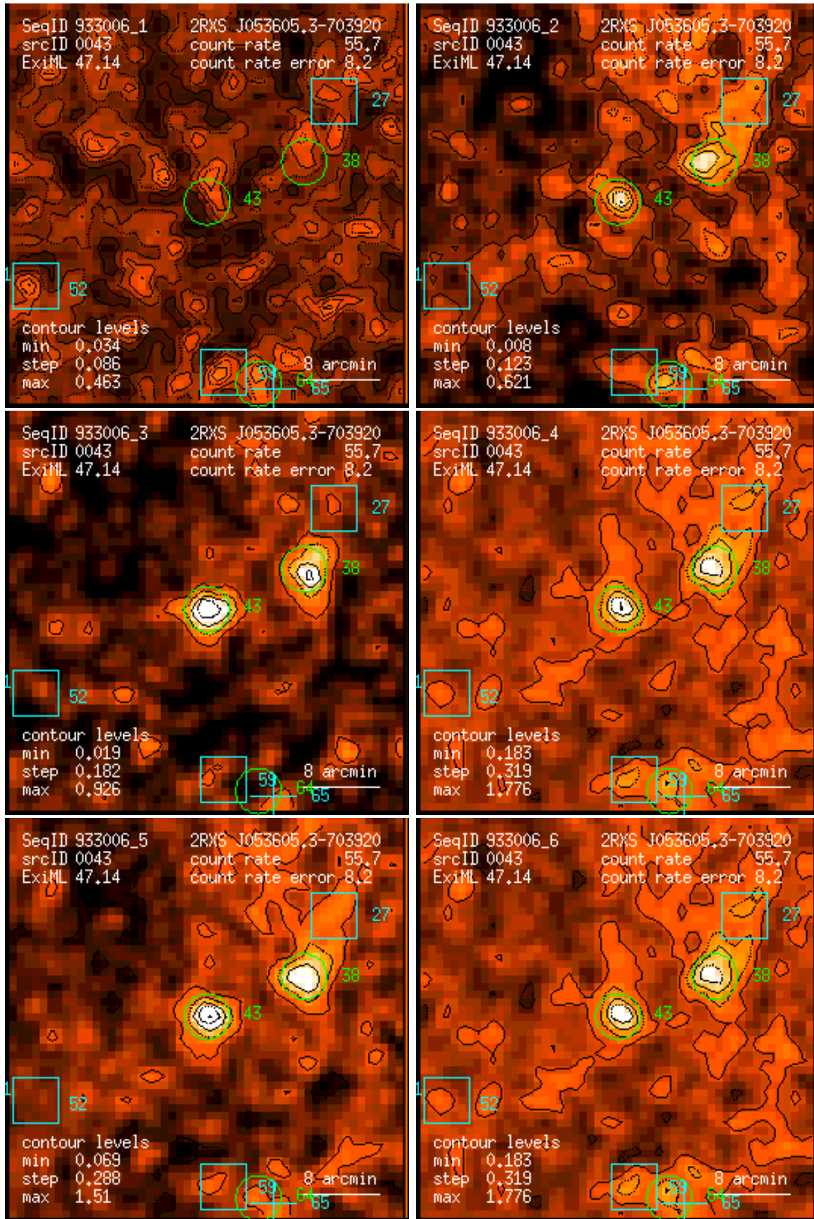
Figure 43: RASS 933006: detection 0043: band rate images, Gaussian filter: (1) PSPC channels 11 – 41, (2) 52 – 90, (3) 91 – 201, (4) 11 – 235, (5) 52 – 201, (6) 11 – 201. Broad band rates in counts/ks. Band rate contour levels in counts/ks/arcmin 2 .
