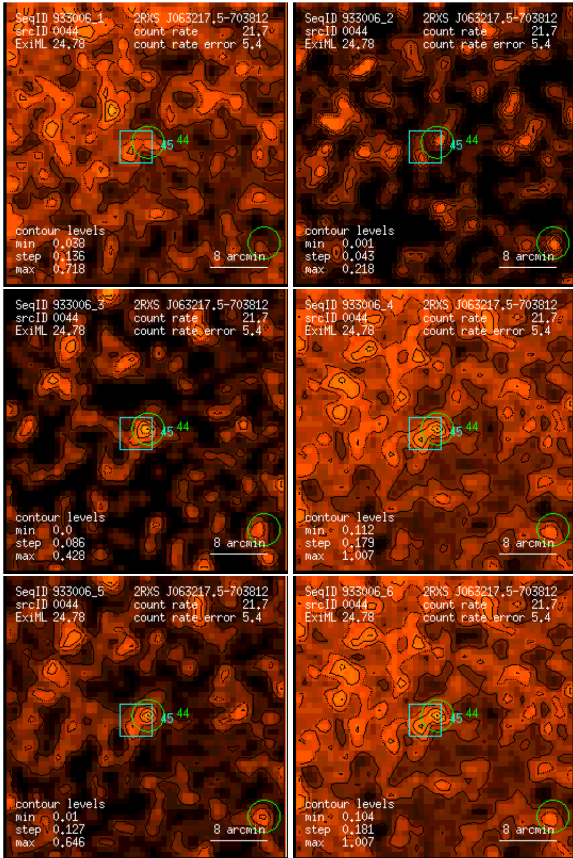
Figure 44: RASS 933006: detection 0044: band rate images, Gaussian filter: (1) PSPC channels 11 – 41, (2) 52 – 90, (3) 91 – 201, (4) 11 – 235, (5) 52 – 201, (6) 11 – 201. Broad band rates in counts/ks. Band rate contour levels in counts/ks/arcmin 2 .
