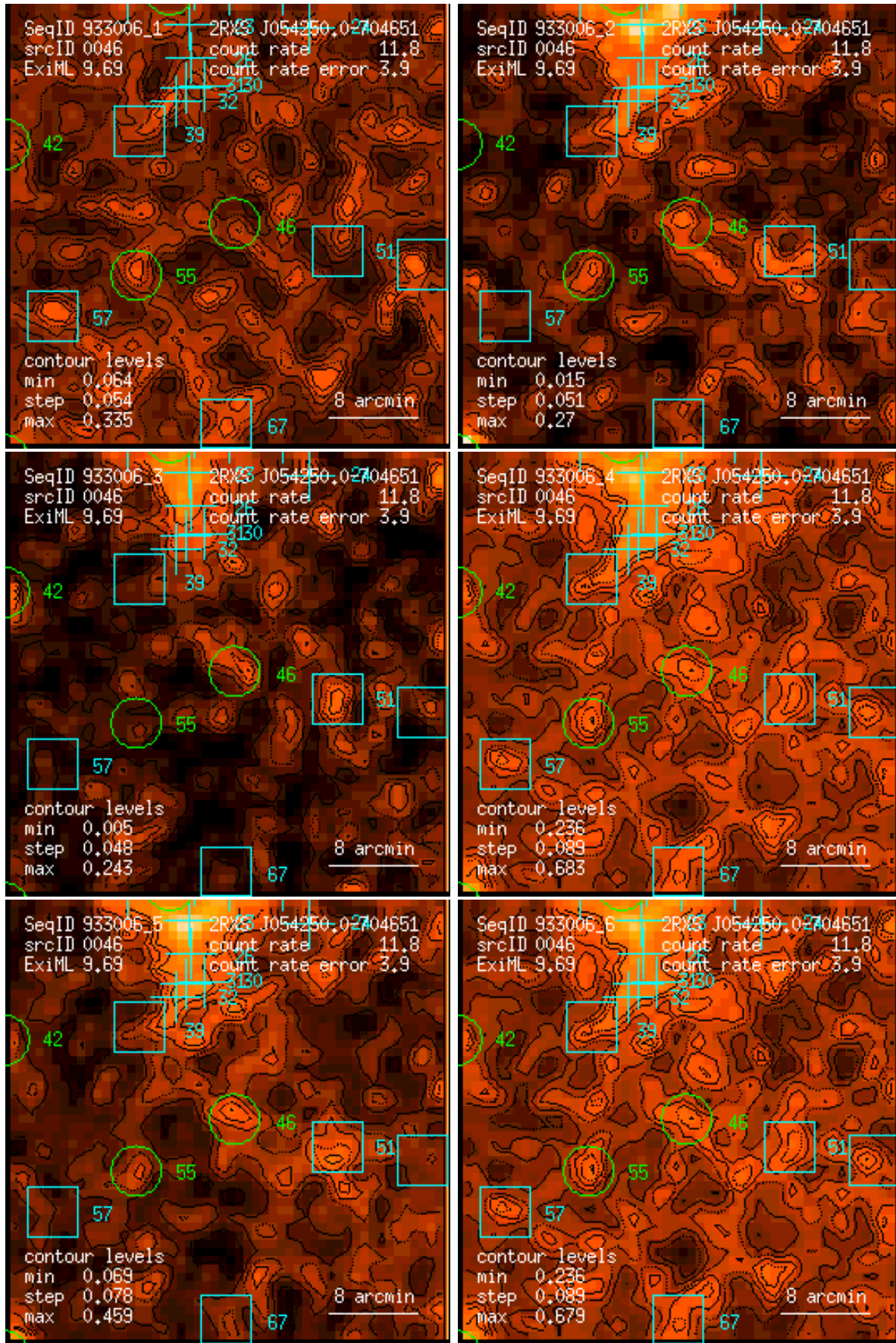
Figure 46: RASS 933006: detection 0046: band rate images, Gaussian filter: (1) PSPC channels 11 – 41, (2) 52 – 90, (3) 91 – 201, (4) 11 – 235, (5) 52 – 201, (6) 11 – 201. Broad band rates in counts/ks. Band rate contour levels in counts/ks/arcmin 2 .
