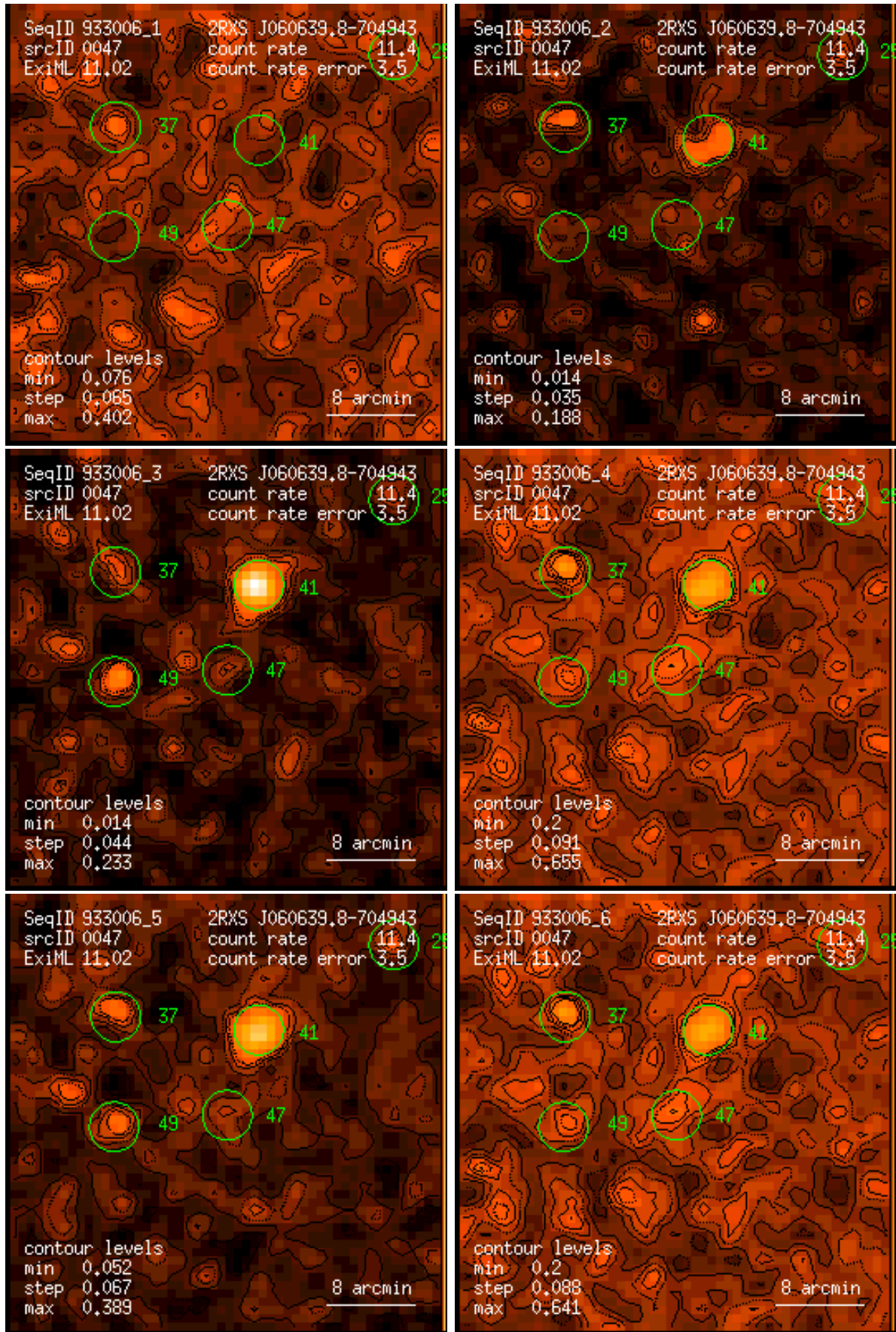
Figure 47: RASS 933006: detection 0047: band rate images, Gaussian filter: (1) PSPC channels 11 – 41, (2) 52 – 90, (3) 91 – 201, (4) 11 – 235, (5) 52 – 201, (6) 11 – 201. Broad band rates in counts/ks. Band rate contour levels in counts/ks/arcmin 2 .
