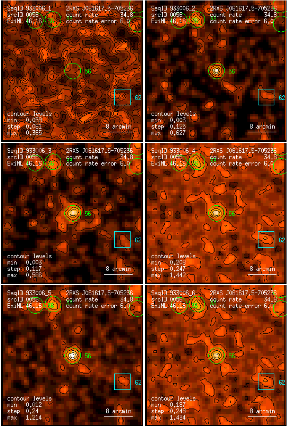
Figure 56: RASS 933006: detection 0056: band rate images, Gaussian filter: (1) PSPC channels 11 – 41, (2) 52 – 90, (3) 91 – 201, (4) 11 – 235, (5) 52 – 201, (6) 11 – 201. Broad band rates in counts/ks. Band rate contour levels in counts/ks/arcmin 2 .
