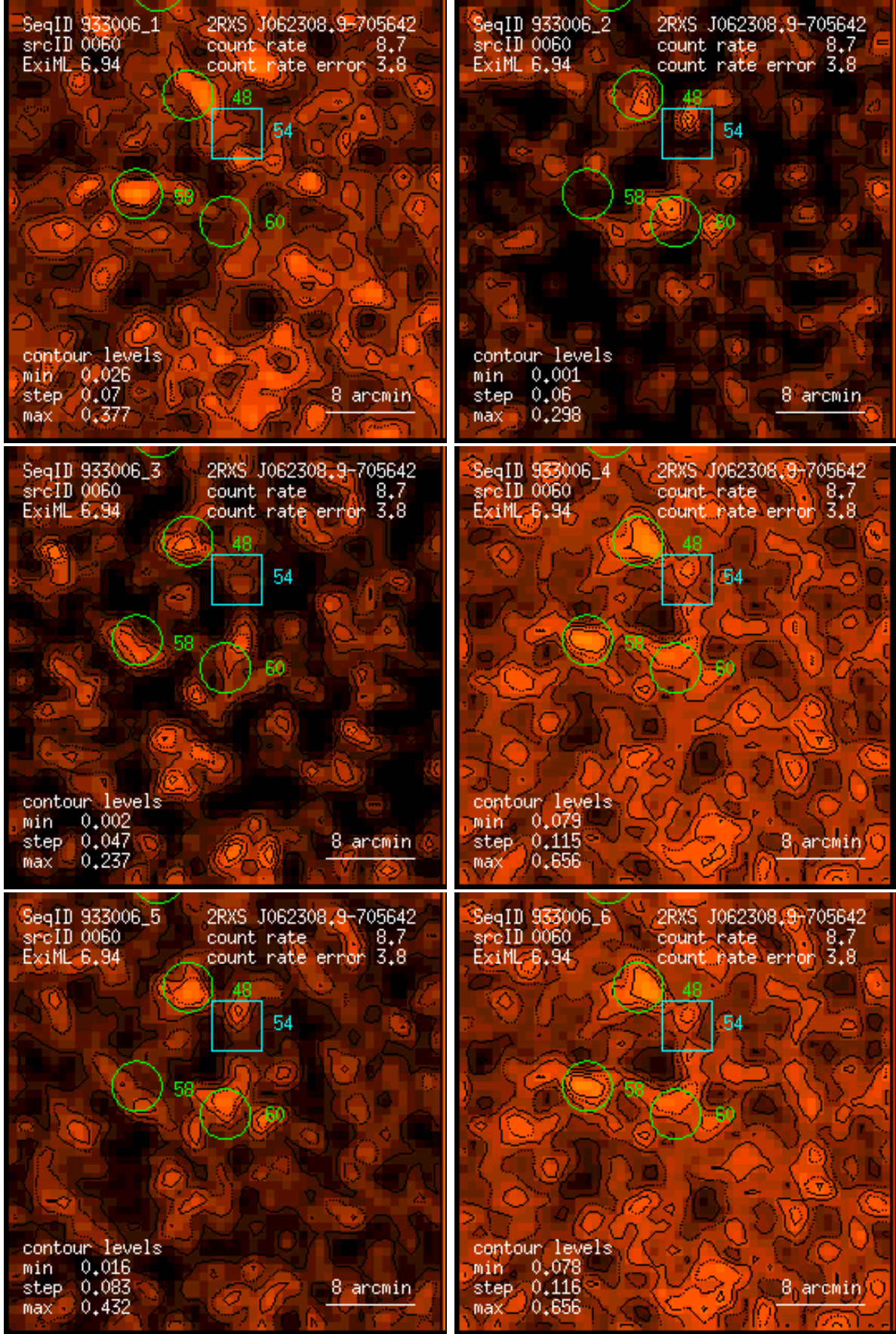
Figure 60: RASS 933006: detection 0060: band rate images, Gaussian filter: (1) PSPC channels 11 – 41, (2) 52 – 90, (3) 91 – 201, (4) 11 – 235, (5) 52 – 201, (6) 11 – 201. Broad band rates in counts/ks. Band rate contour levels in counts/ks/arcmin 2 .
