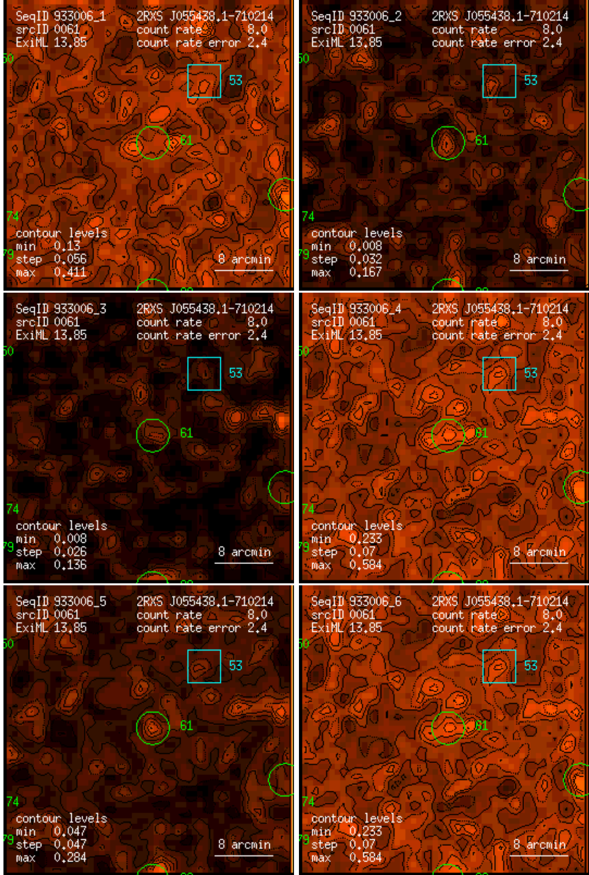
Figure 61: RASS 933006: detection 0061: band rate images, Gaussian filter: (1) PSPC channels 11 – 41, (2) 52 – 90, (3) 91 – 201, (4) 11 – 235, (5) 52 – 201, (6) 11 – 201. Broad band rates in counts/ks. Band rate contour levels in counts/ks/arcmin 2 .
