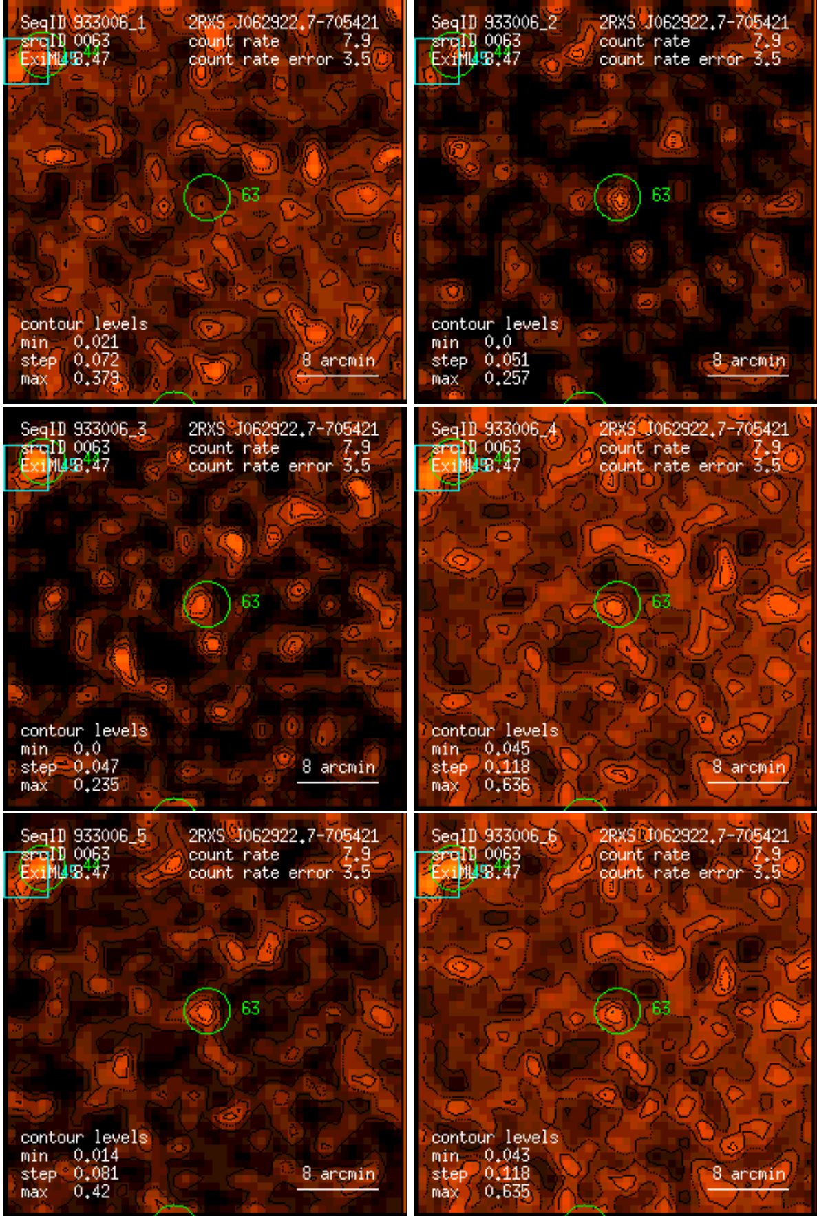
Figure 63: RASS 933006: detection 0063: band rate images, Gaussian filter: (1) PSPC channels 11 – 41, (2) 52 – 90, (3) 91 – 201, (4) 11 – 235, (5) 52 – 201, (6) 11 – 201. Broad band rates in counts/ks. Band rate contour levels in counts/ks/arcmin 2 .
