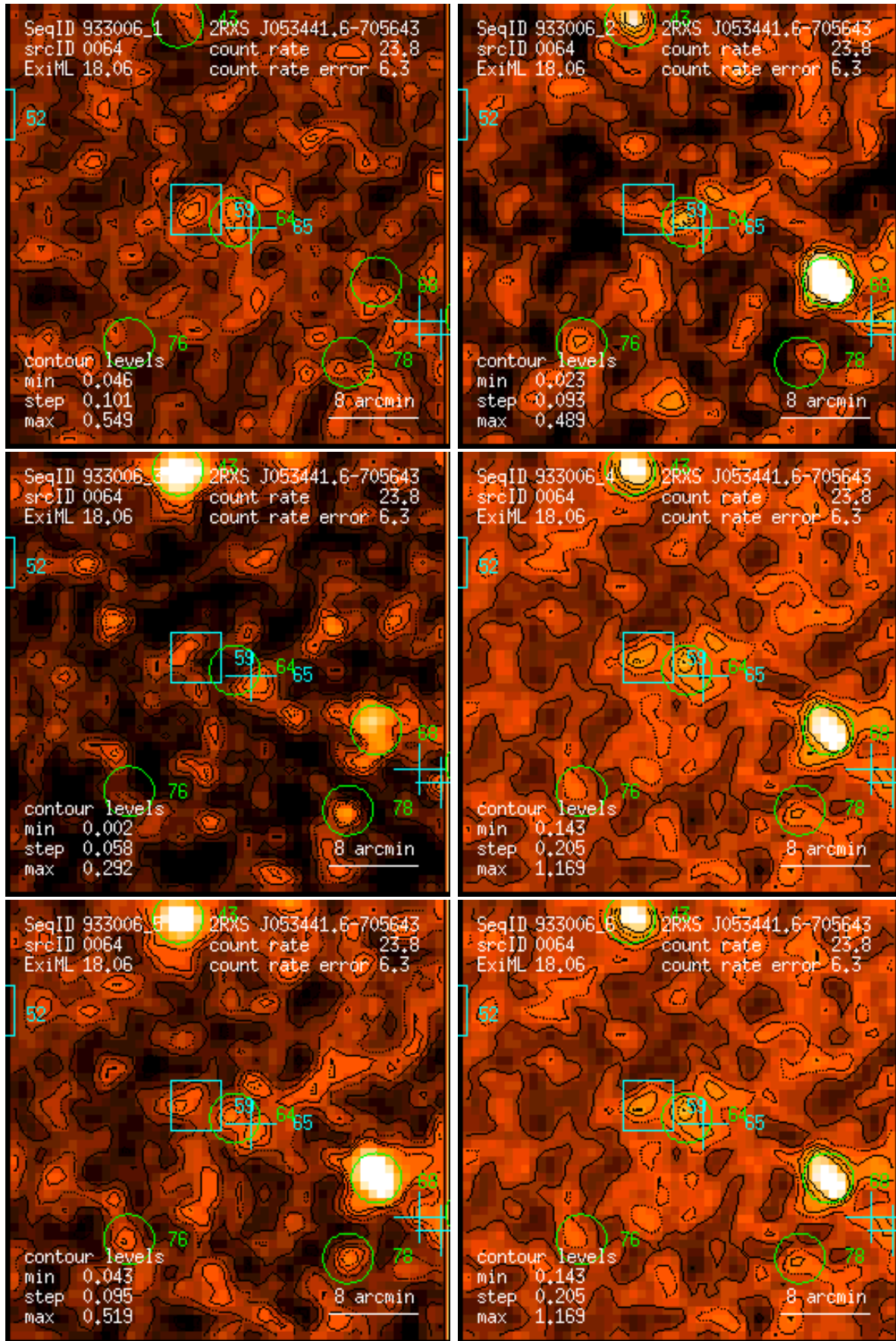
Figure 64: RASS 933006: detection 0064: band rate images, Gaussian filter: (1) PSPC channels 11 – 41, (2) 52 – 90, (3) 91 – 201, (4) 11 – 235, (5) 52 – 201, (6) 11 – 201. Broad band rates in counts/ks. Band rate contour levels in counts/ks/arcmin 2 .
