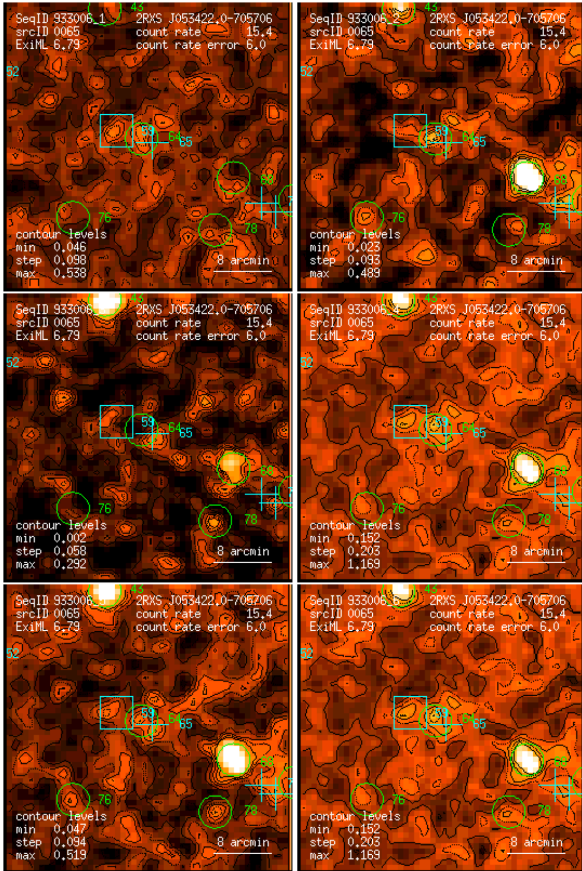
Figure 65: RASS 933006: detection 0065: band rate images, Gaussian filter: (1) PSPC channels 11 – 41, (2) 52 – 90, (3) 91 – 201, (4) 11 – 235, (5) 52 – 201, (6) 11 – 201. Broad band rates in counts/ks. Band rate contour levels in counts/ks/arcmin 2 .
