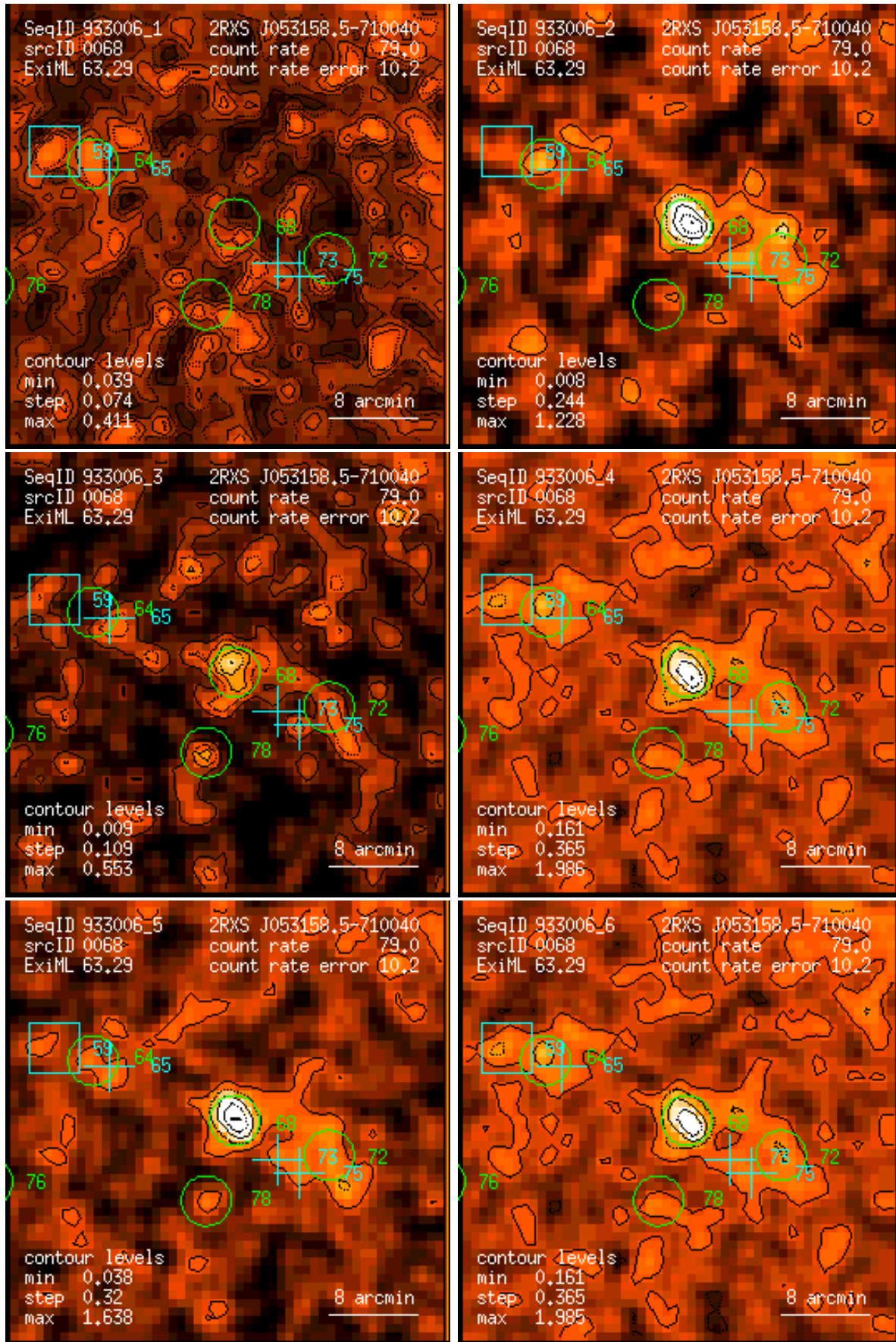
Figure 68: RASS 933006: detection 0068: band rate images, Gaussian filter: (1) PSPC channels 11 – 41, (2) 52 – 90, (3) 91 – 201, (4) 11 – 235, (5) 52 – 201, (6) 11 – 201. Broad band rates in counts/ks. Band rate contour levels in counts/ks/arcmin 2 .
