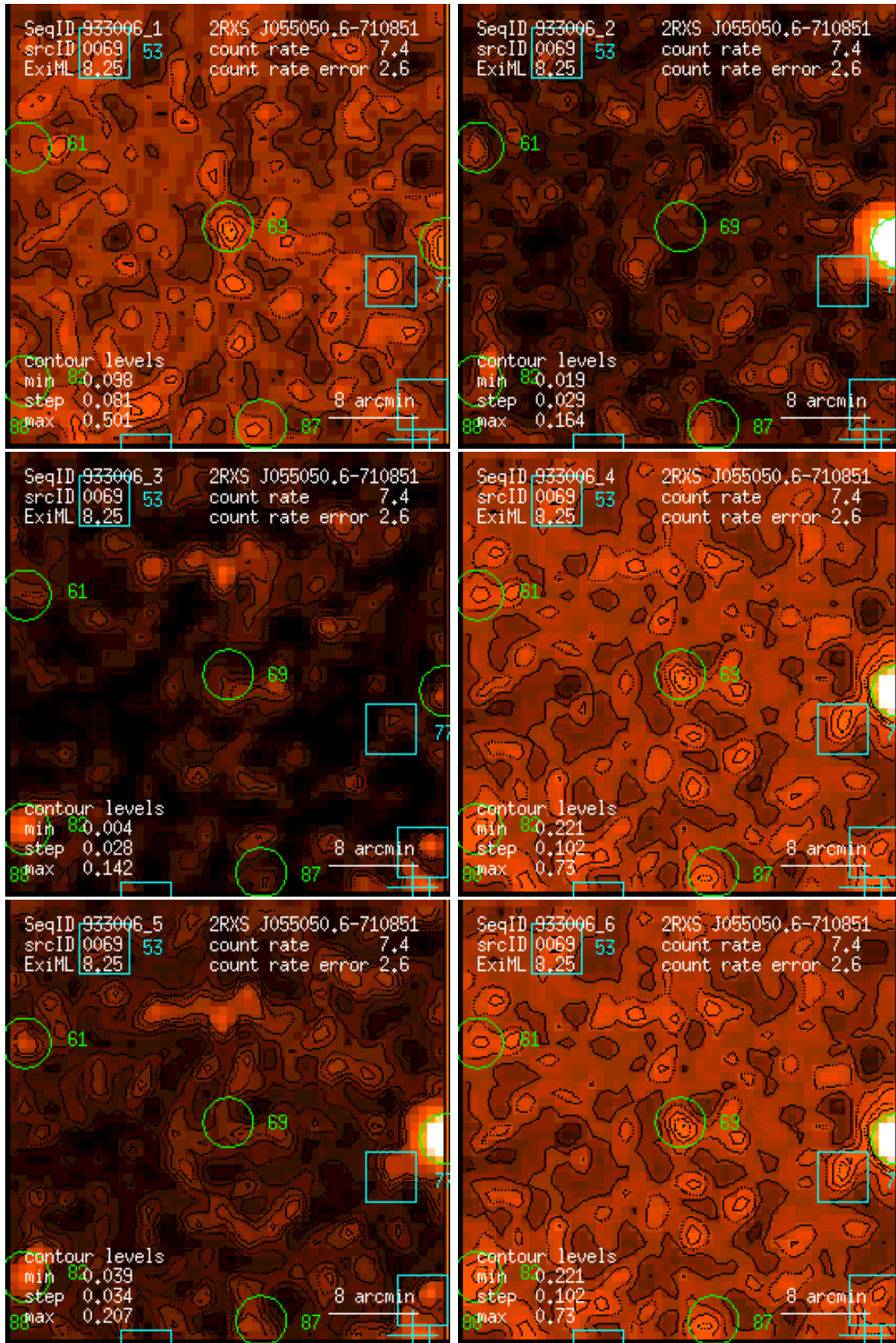
Figure 69: RASS 933006: detection 0069: band rate images, Gaussian filter: (1) PSPC channels 11 – 41, (2) 52 – 90, (3) 91 – 201, (4) 11 – 235, (5) 52 – 201, (6) 11 – 201. Broad band rates in counts/ks. Band rate contour levels in counts/ks/arcmin 2 .
