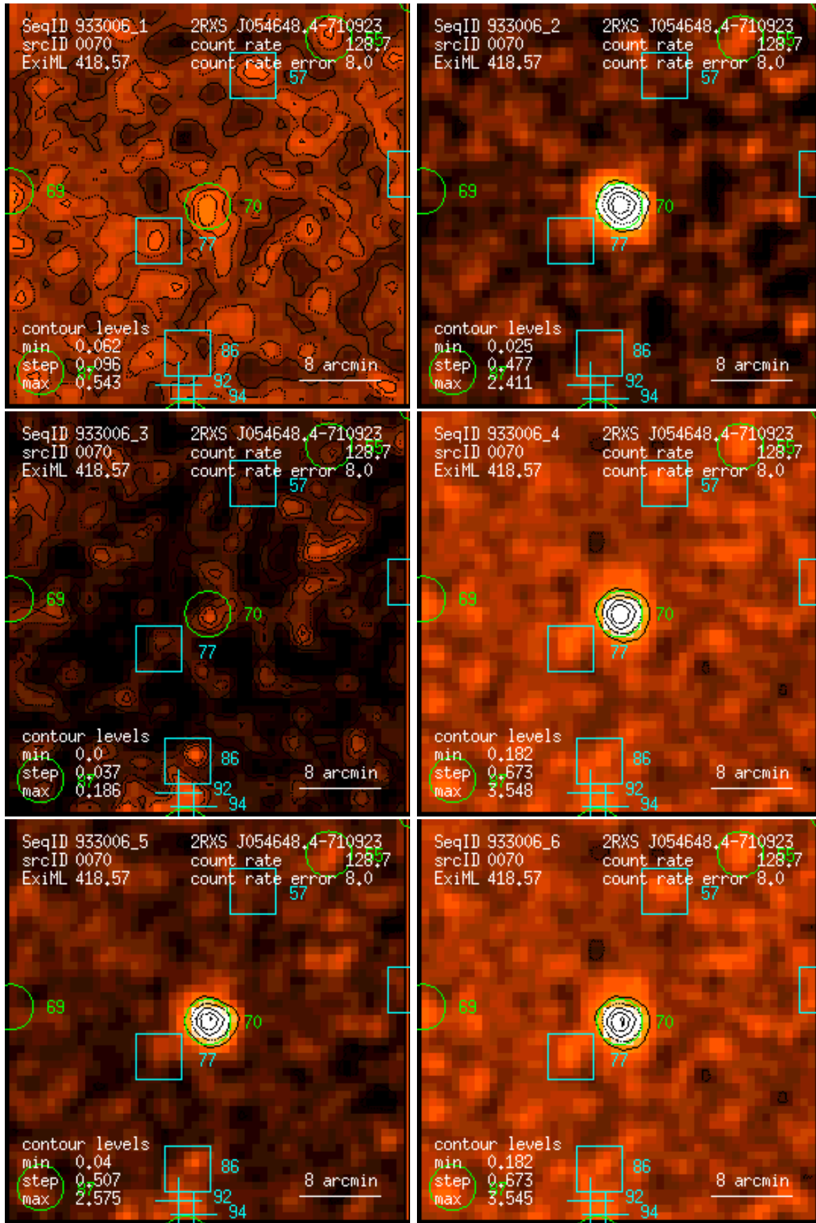
Figure 70: RASS 933006: detection 0070: band rate images, Gaussian filter: (1) PSPC channels 11 – 41, (2) 52 – 90, (3) 91 – 201, (4) 11 – 235, (5) 52 – 201, (6) 11 – 201. Broad band rates in counts/ks. Band rate contour levels in counts/ks/arcmin 2 .
