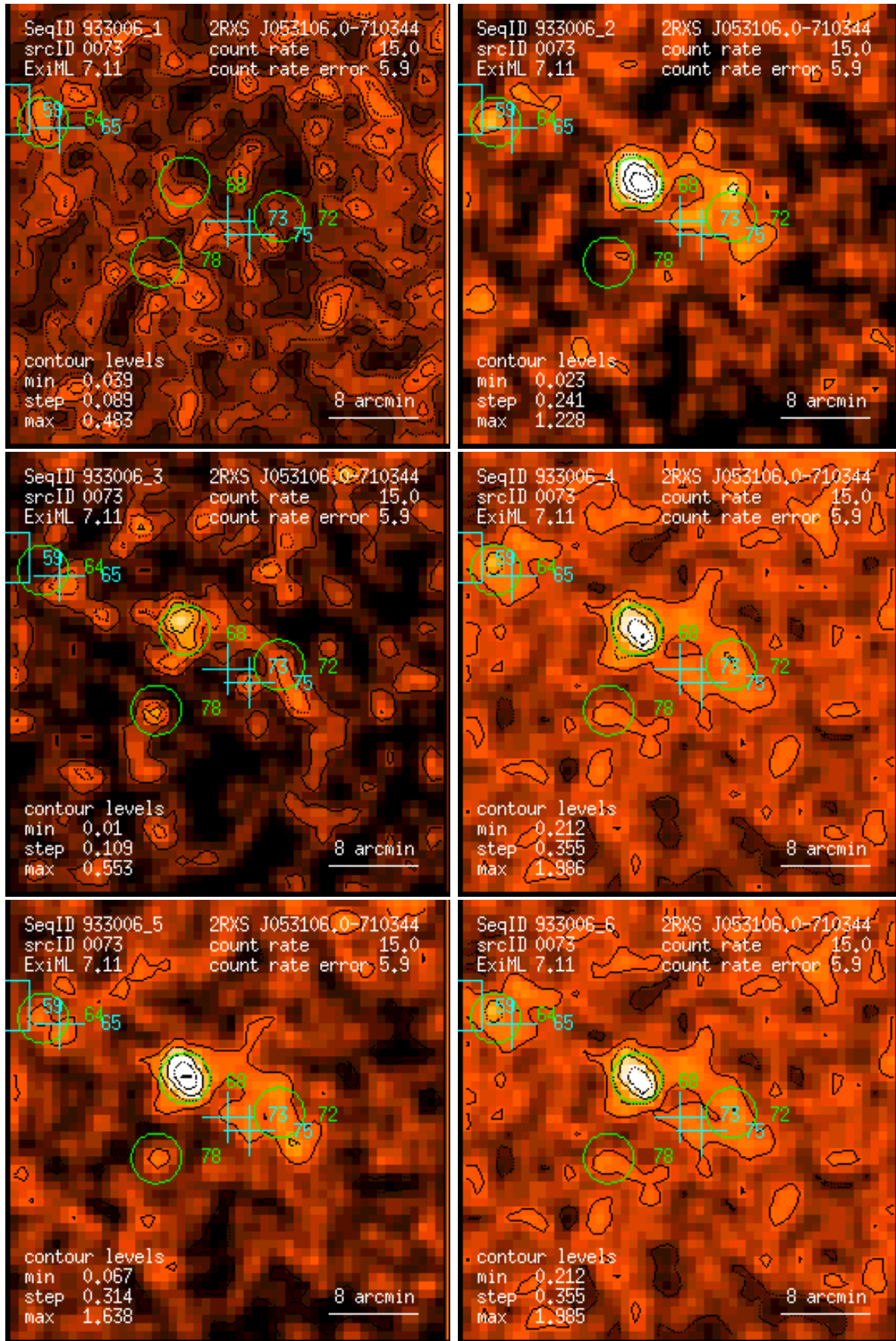
Figure 73: RASS 933006: detection 0073: band rate images, Gaussian filter: (1) PSPC channels 11 – 41, (2) 52 – 90, (3) 91 – 201, (4) 11 – 235, (5) 52 – 201, (6) 11 – 201. Broad band rates in counts/ks. Band rate contour levels in counts/ks/arcmin 2 .
