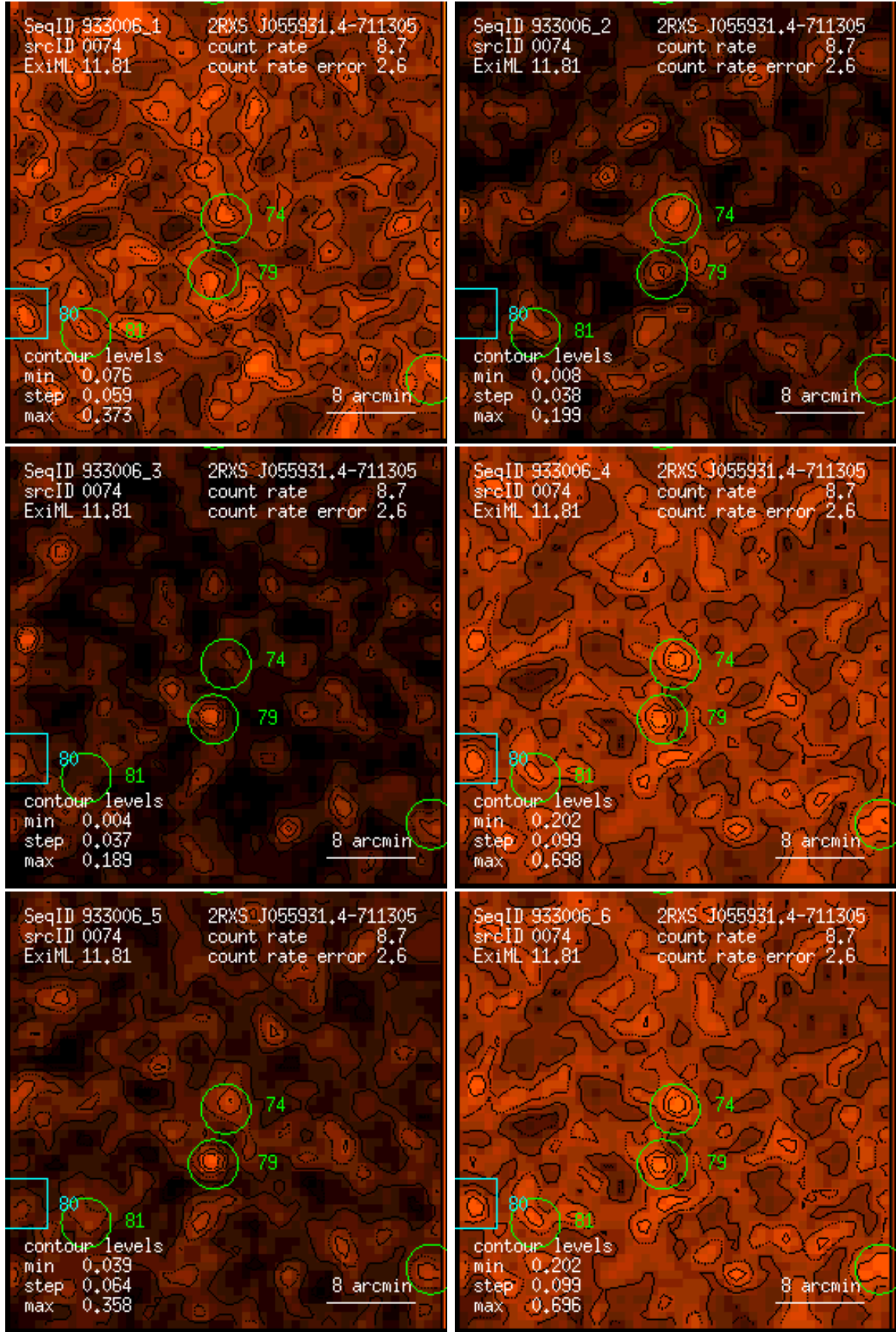
Figure 74: RASS 933006: detection 0074: band rate images, Gaussian filter: (1) PSPC channels 11 – 41, (2) 52 – 90, (3) 91 – 201, (4) 11 – 235, (5) 52 – 201, (6) 11 – 201. Broad band rates in counts/ks. Band rate contour levels in counts/ks/arcmin 2 .
