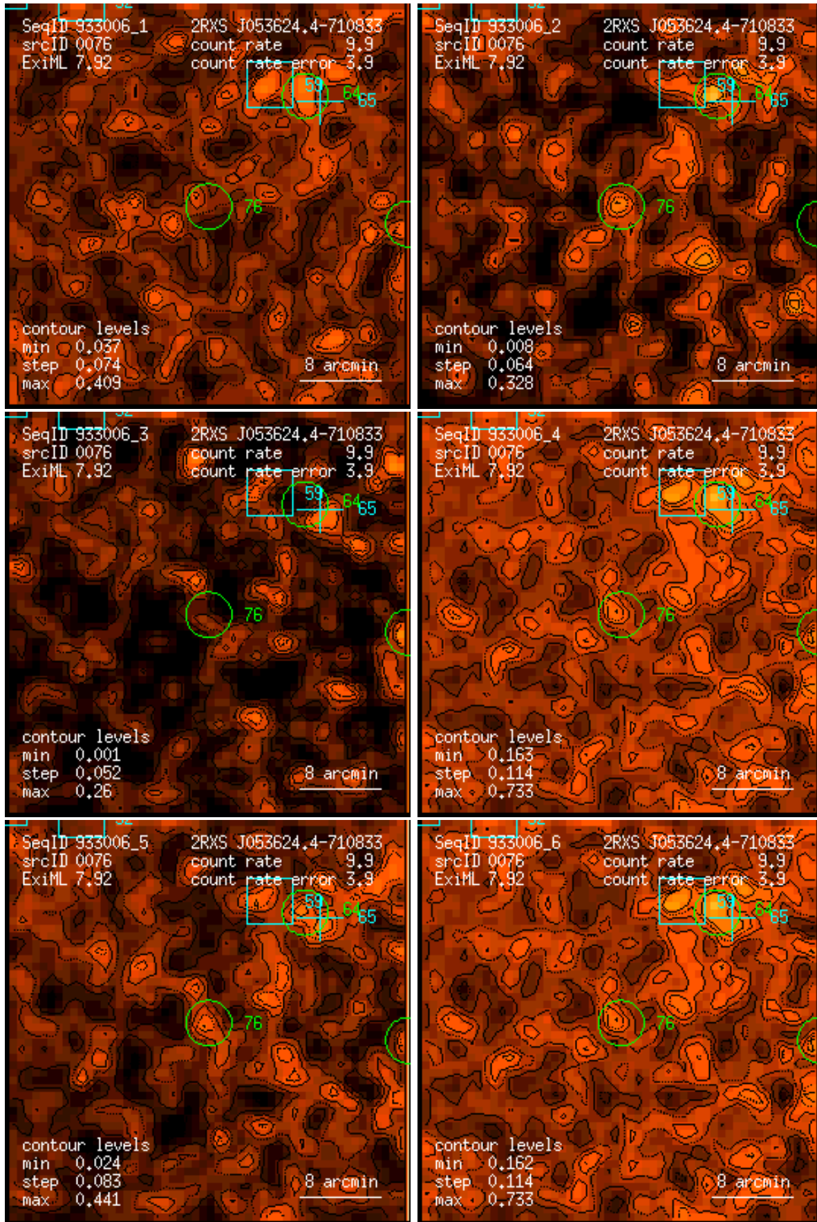
Figure 76: RASS 933006: detection 0076: band rate images, Gaussian filter: (1) PSPC channels 11 – 41, (2) 52 – 90, (3) 91 – 201, (4) 11 – 235, (5) 52 – 201, (6) 11 – 201. Broad band rates in counts/ks. Band rate contour levels in counts/ks/arcmin 2 .
