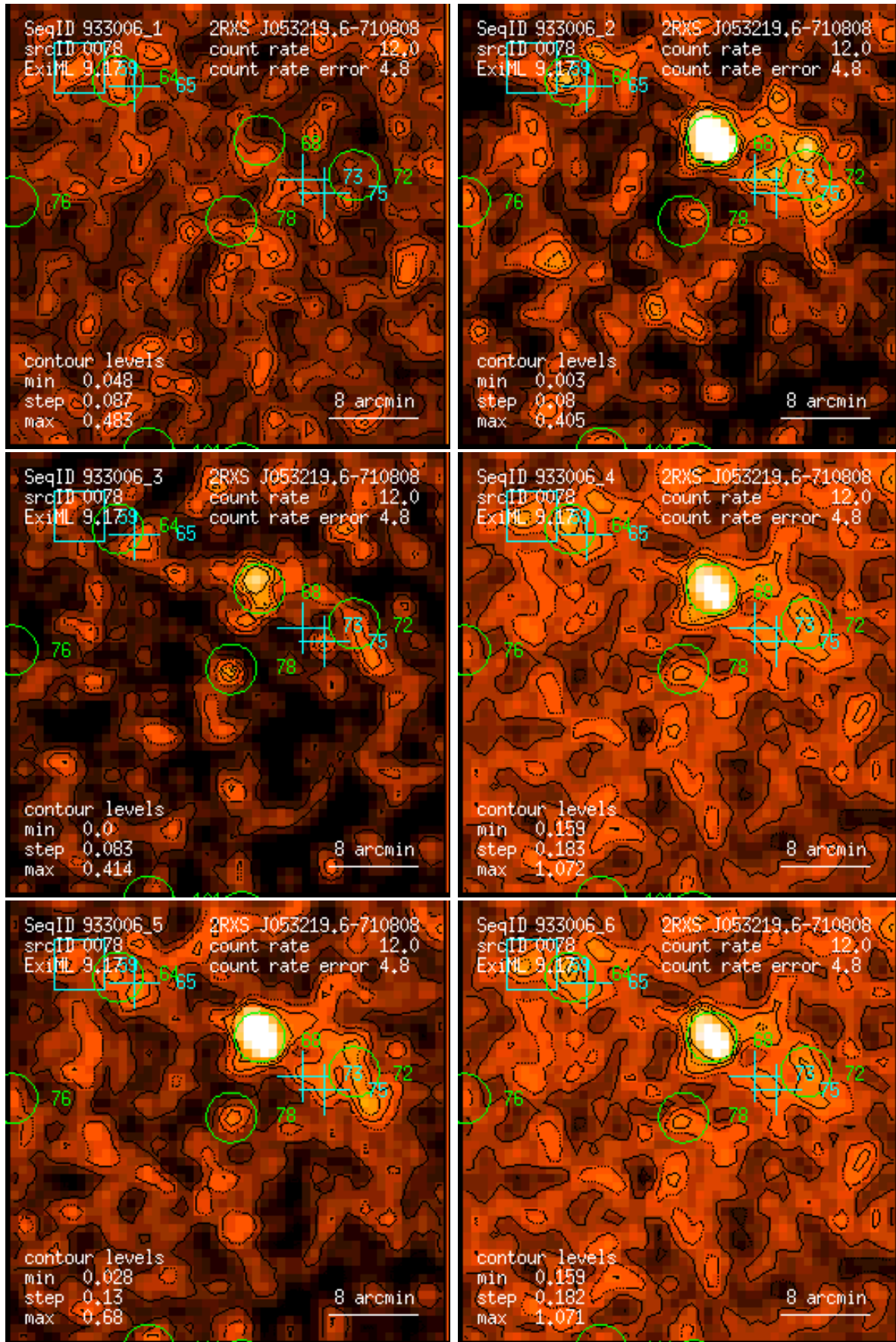
Figure 78: RASS 933006: detection 0078: band rate images, Gaussian filter: (1) PSPC channels 11 – 41, (2) 52 – 90, (3) 91 – 201, (4) 11 – 235, (5) 52 – 201, (6) 11 – 201. Broad band rates in counts/ks. Band rate contour levels in counts/ks/arcmin 2 .
