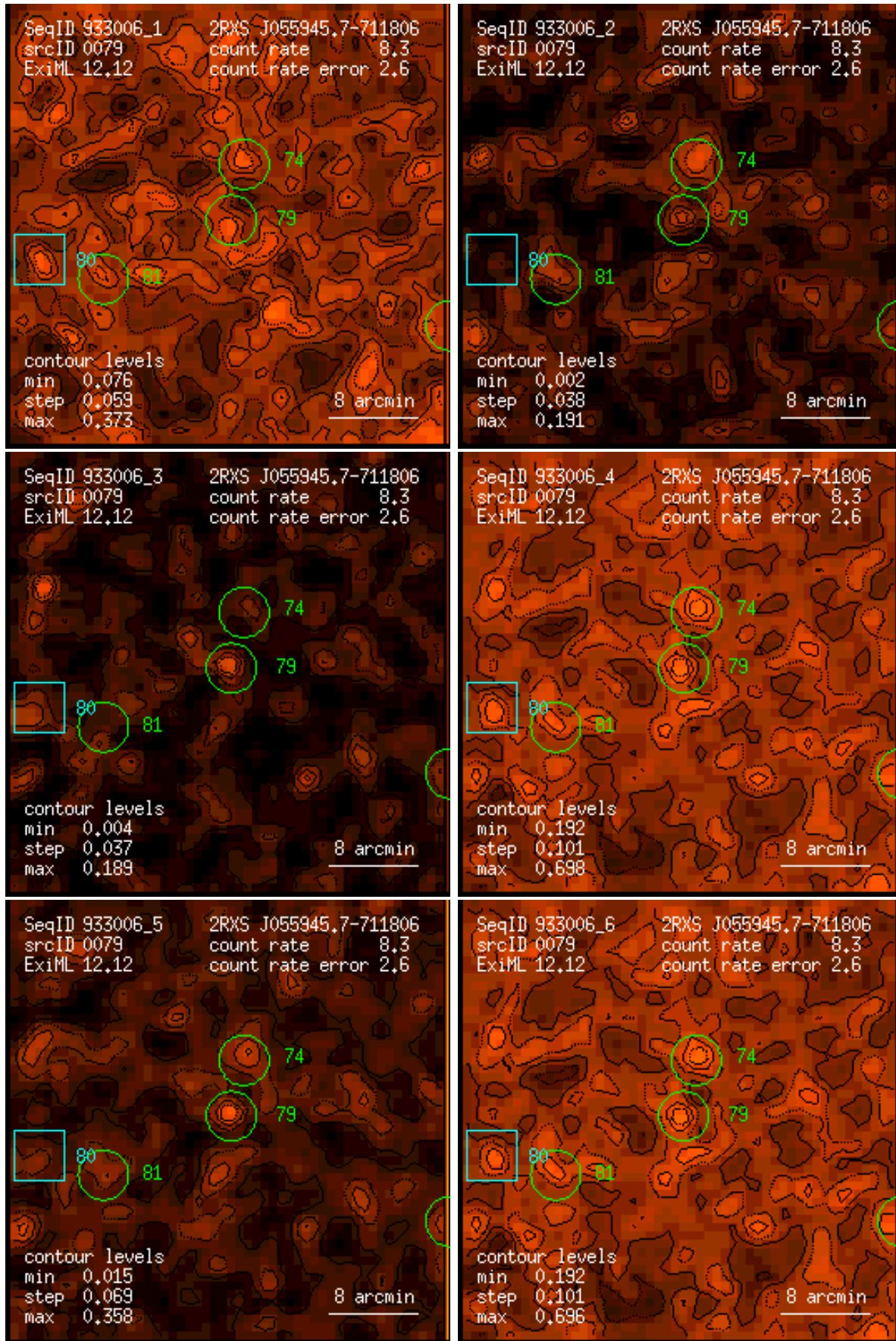
Figure 79: RASS 933006: detection 0079: band rate images, Gaussian filter: (1) PSPC channels 11 – 41, (2) 52 – 90, (3) 91 – 201, (4) 11 – 235, (5) 52 – 201, (6) 11 – 201. Broad band rates in counts/ks. Band rate contour levels in counts/ks/arcmin 2 .
