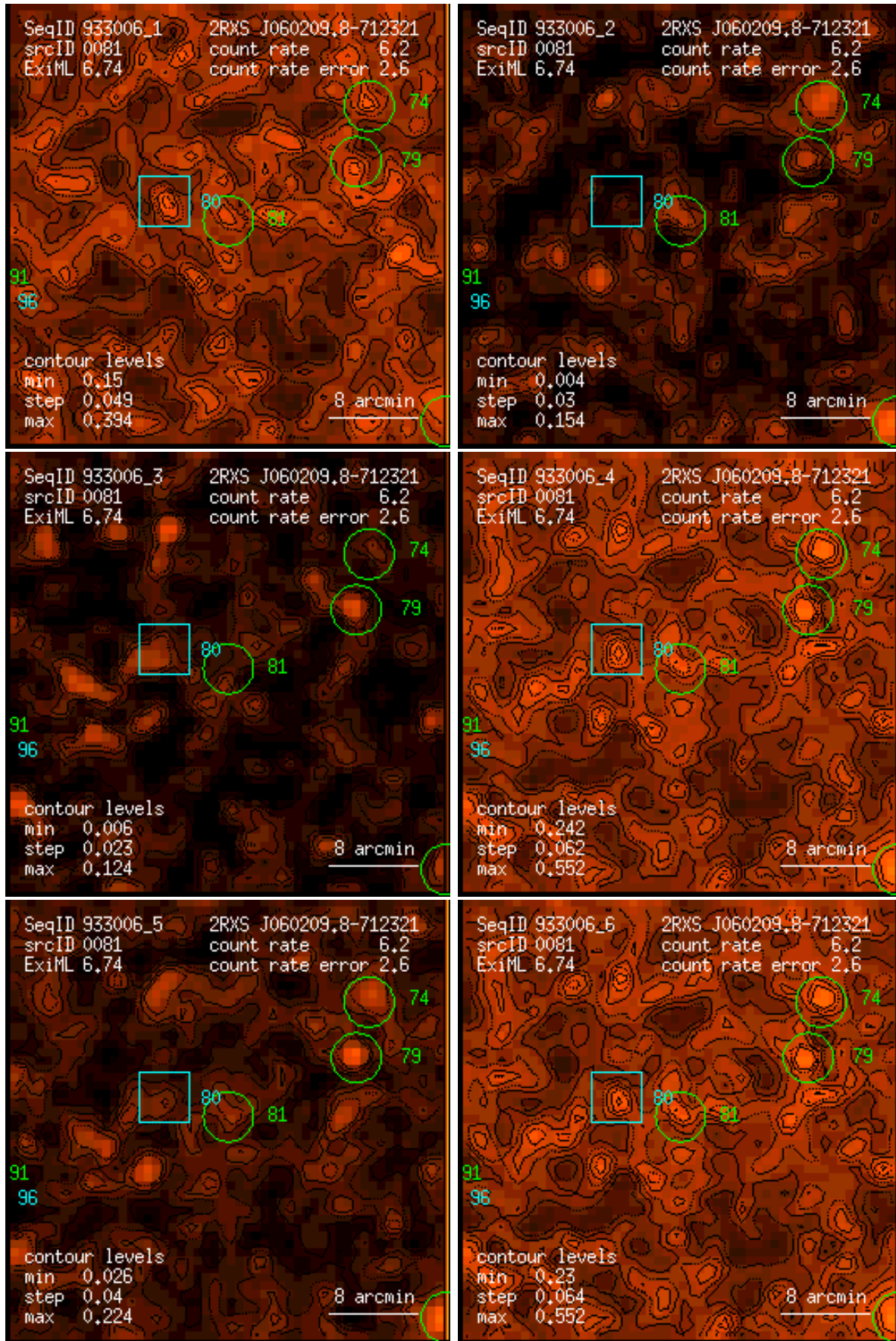
Figure 81: RASS 933006: detection 0081: band rate images, Gaussian filter: (1) PSPC channels 11 – 41, (2) 52 – 90, (3) 91 – 201, (4) 11 – 235, (5) 52 – 201, (6) 11 – 201. Broad band rates in counts/ks. Band rate contour levels in counts/ks/arcmin 2 .
