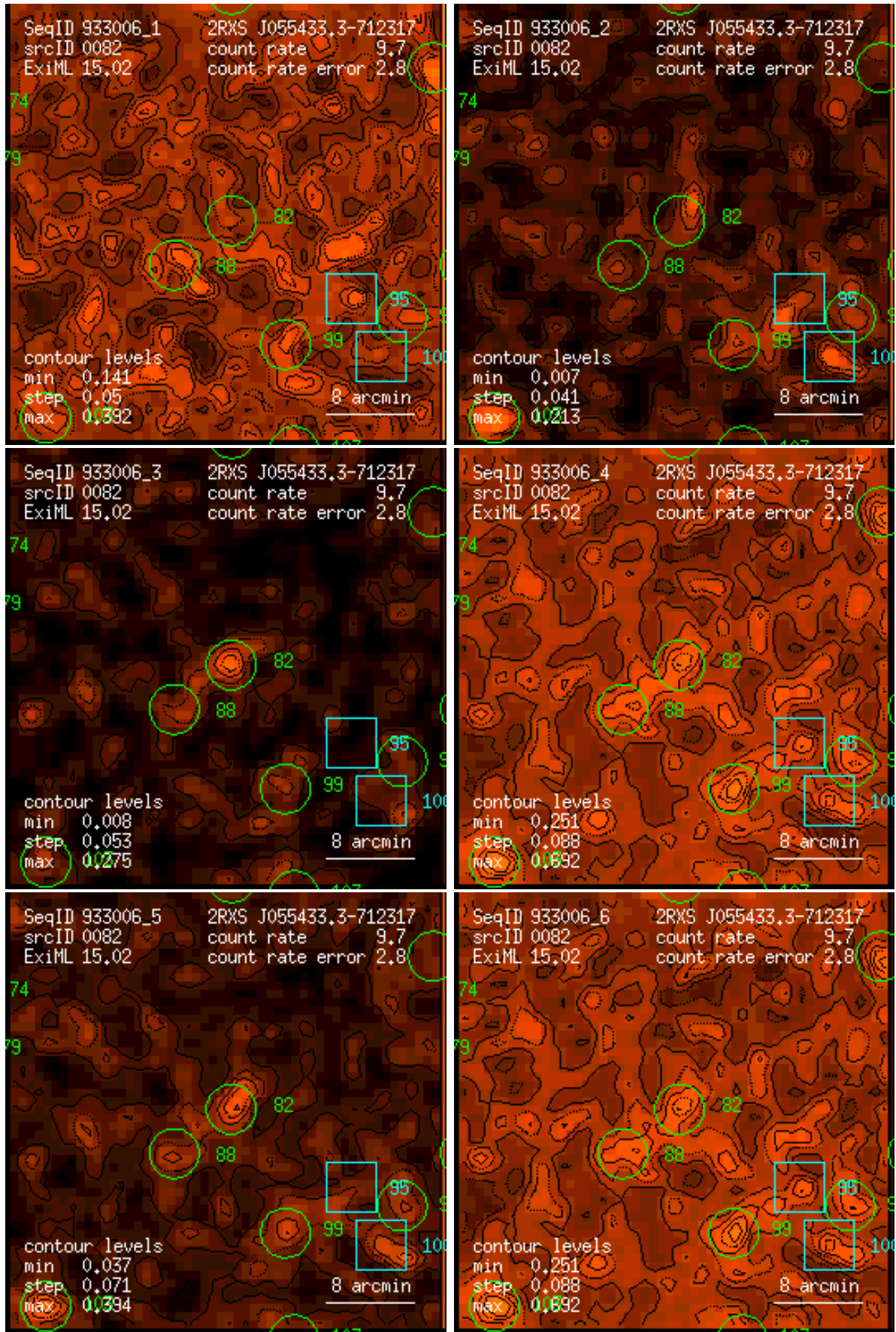
Figure 82: RASS 933006: detection 0082: band rate images, Gaussian filter: (1) PSPC channels 11 – 41, (2) 52 – 90, (3) 91 – 201, (4) 11 – 235, (5) 52 – 201, (6) 11 – 201. Broad band rates in counts/ks. Band rate contour levels in counts/ks/arcmin 2 .
