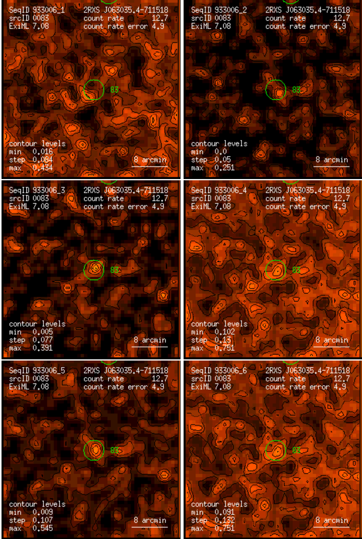
Figure 83: RASS 933006: detection 0083: band rate images, Gaussian filter: (1) PSPC channels 11 – 41, (2) 52 – 90, (3) 91 – 201, (4) 11 – 235, (5) 52 – 201, (6) 11 – 201. Broad band rates in counts/ks. Band rate contour levels in counts/ks/arcmin 2 .
