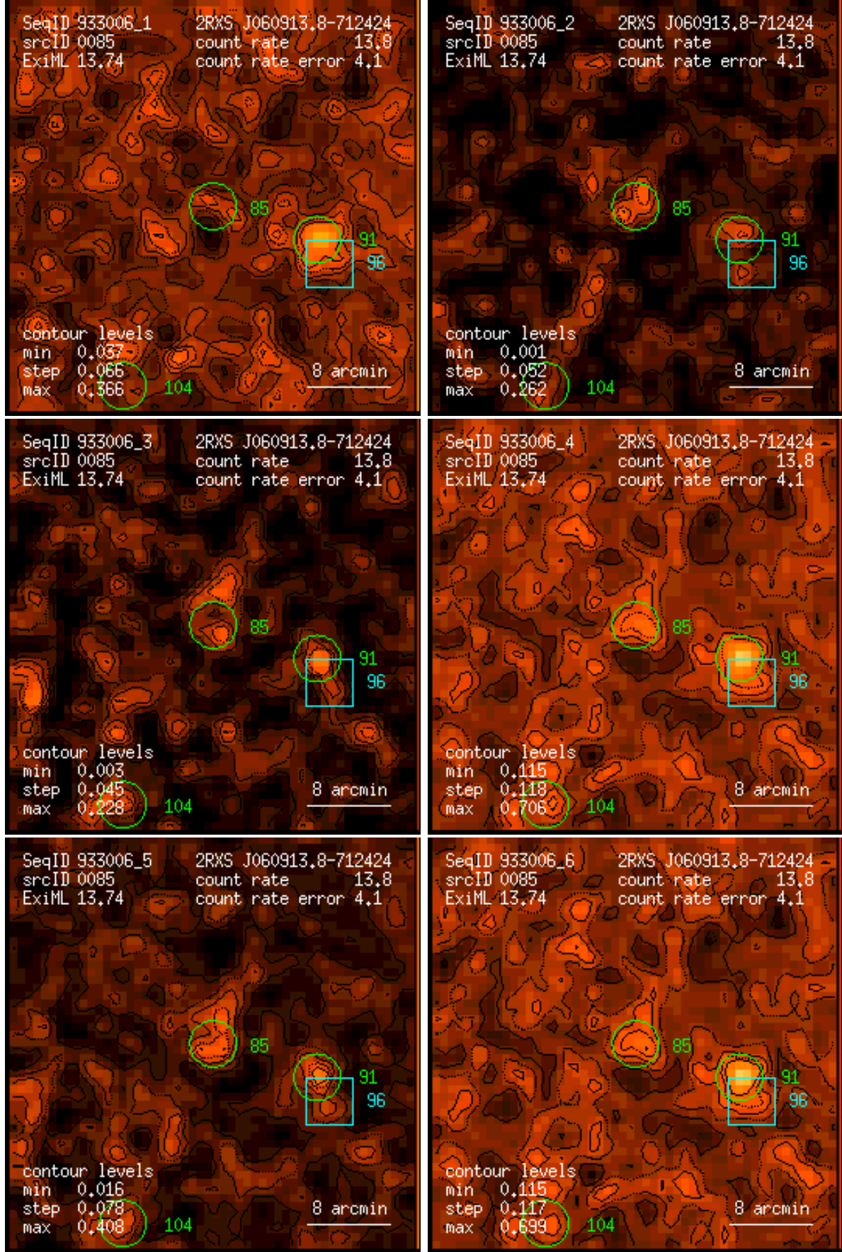
Figure 85: RASS 933006: detection 0085: band rate images, Gaussian filter: (1) PSPC channels 11 – 41, (2) 52 – 90, (3) 91 – 201, (4) 11 – 235, (5) 52 – 201, (6) 11 – 201. Broad band rates in counts/ks. Band rate contour levels in counts/ks/arcmin 2 .
