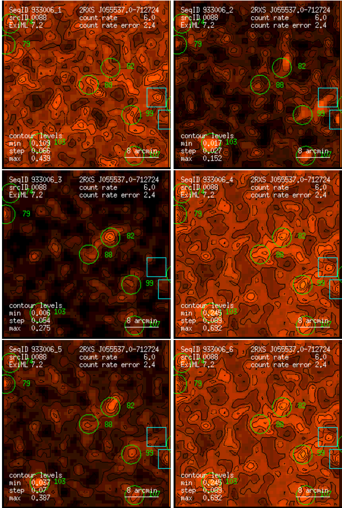
Figure 88: RASS 933006: detection 0088: band rate images, Gaussian filter: (1) PSPC channels 11 – 41, (2) 52 – 90, (3) 91 – 201, (4) 11 – 235, (5) 52 – 201, (6) 11 – 201. Broad band rates in counts/ks. Band rate contour levels in counts/ks/arcmin 2 .
