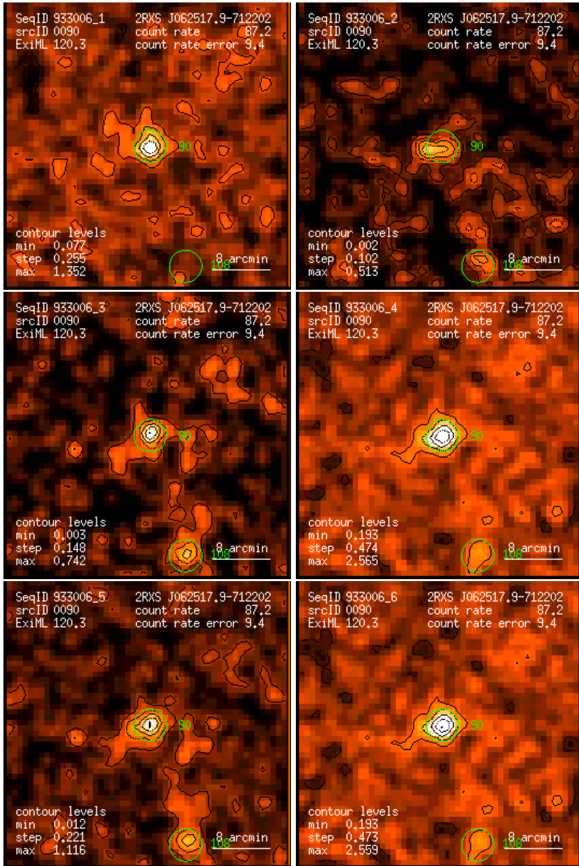
Figure 90: RASS 933006: detection 0090: band rate images, Gaussian filter: (1) PSPC channels 11 – 41, (2) 52 – 90, (3) 91 – 201, (4) 11 – 235, (5) 52 – 201, (6) 11 – 201. Broad band rates in counts/ks. Band rate contour levels in counts/ks/arcmin 2 .
