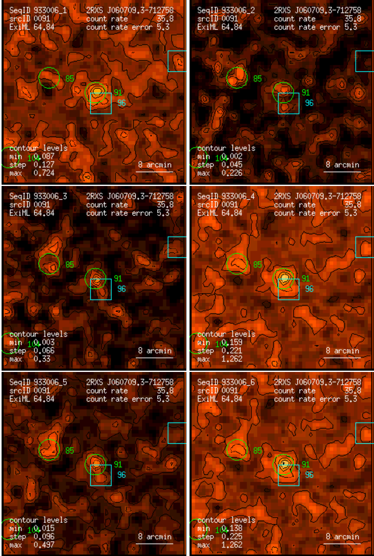
Figure 91: RASS 933006: detection 0091: band rate images, Gaussian filter: (1) PSPC channels 11 – 41, (2) 52 – 90, (3) 91 – 201, (4) 11 – 235, (5) 52 – 201, (6) 11 – 201. Broad band rates in counts/ks. Band rate contour levels in counts/ks/arcmin 2 .
