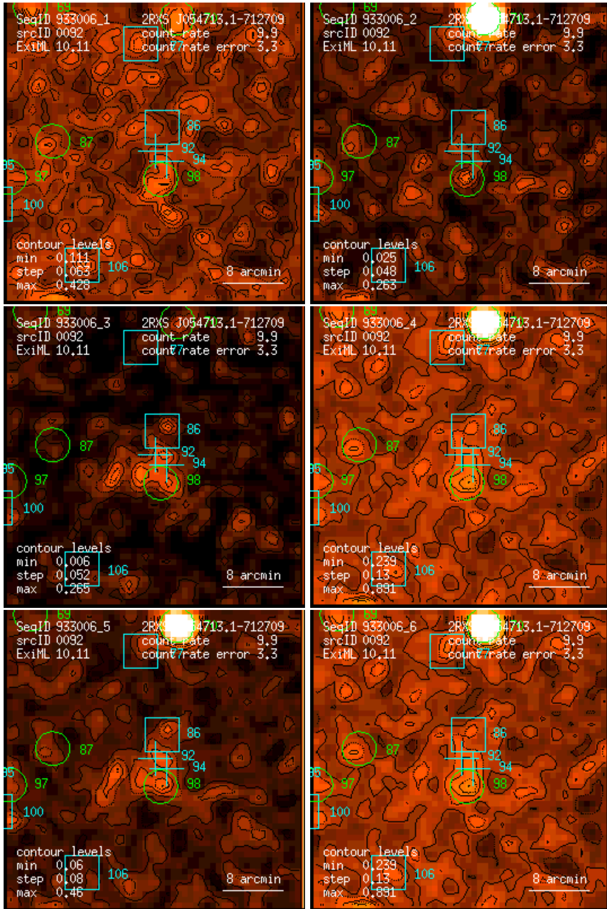
Figure 92: RASS 933006: detection 0092: band rate images, Gaussian filter: (1) PSPC channels 11 – 41, (2) 52 – 90, (3) 91 – 201, (4) 11 – 235, (5) 52 – 201, (6) 11 – 201. Broad band rates in counts/ks. Band rate contour levels in counts/ks/arcmin 2 .
