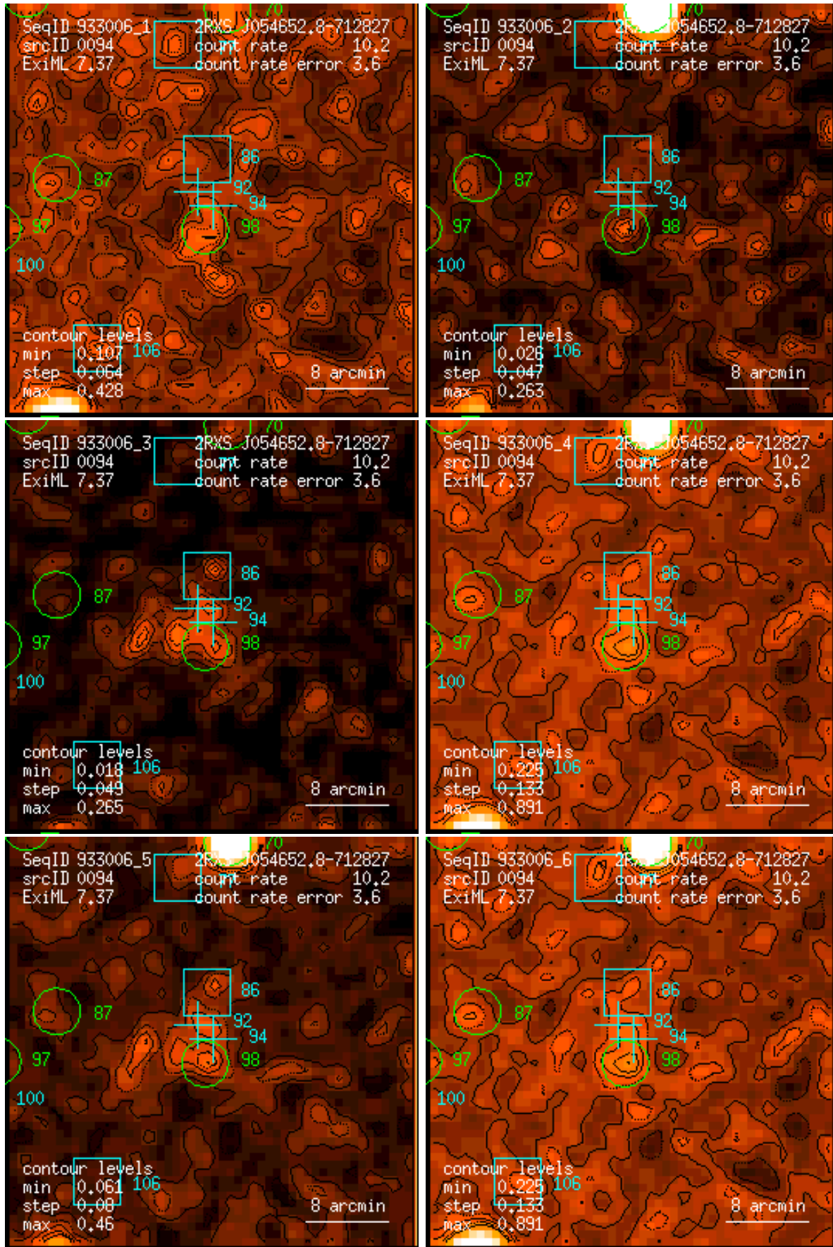
Figure 94: RASS 933006: detection 0094: band rate images, Gaussian filter: (1) PSPC channels 11 – 41, (2) 52 – 90, (3) 91 – 201, (4) 11 – 235, (5) 52 – 201, (6) 11 – 201. Broad band rates in counts/ks. Band rate contour levels in counts/ks/arcmin 2 .
