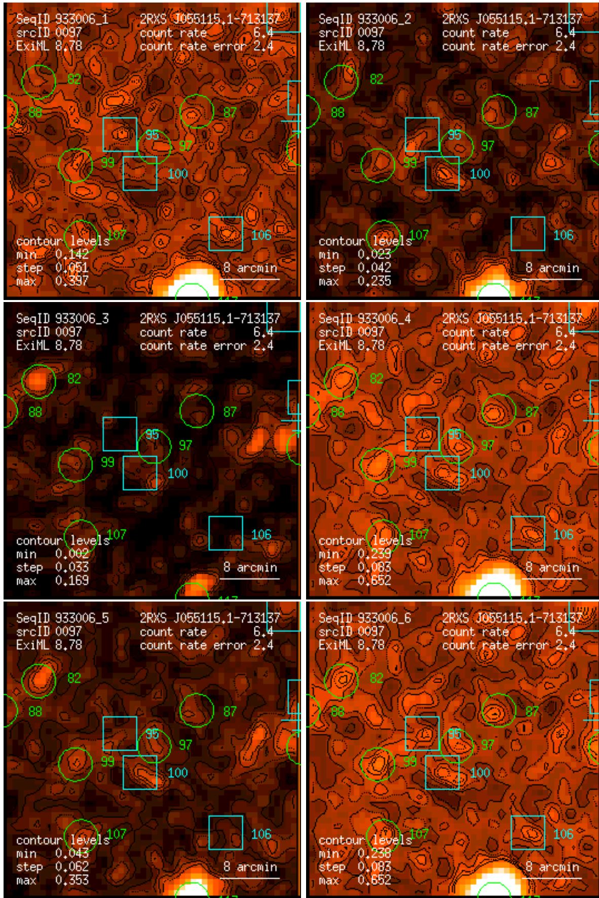
Figure 97: RASS 933006: detection 0097: band rate images, Gaussian filter: (1) PSPC channels 11 – 41, (2) 52 – 90, (3) 91 – 201, (4) 11 – 235, (5) 52 – 201, (6) 11 – 201. Broad band rates in counts/ks. Band rate contour levels in counts/ks/arcmin 2 .
